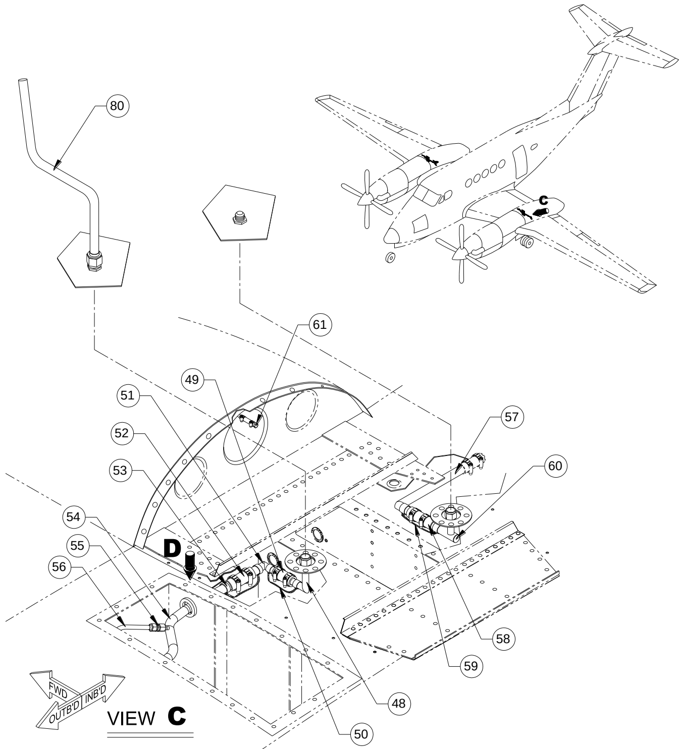
FIGURE 20-13 - FUEL SYSTEM INSTALLATION, ST120 SHEET 3 OF 4
