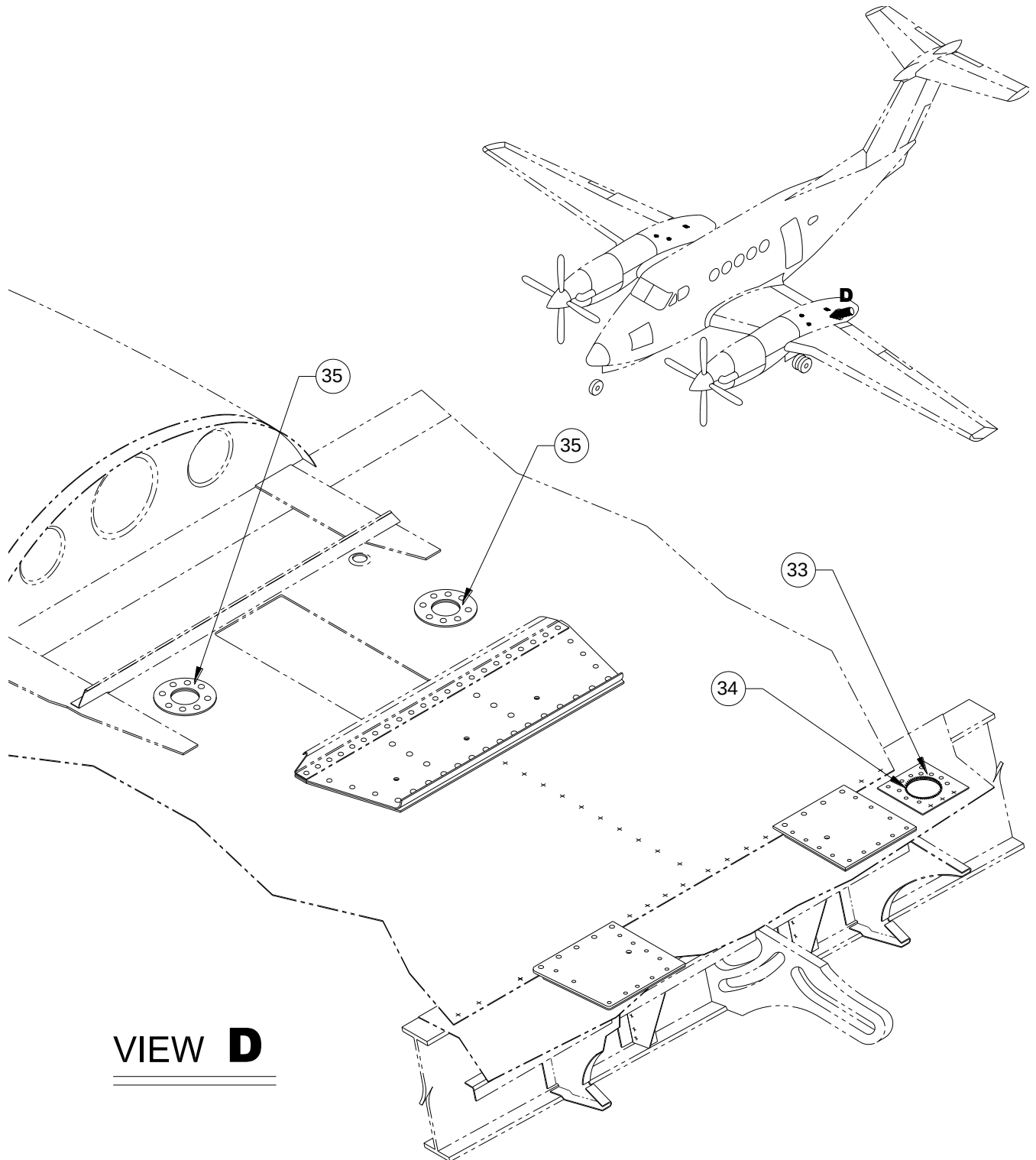
FIGURE 10-10 - SADDLE TANKS INSTALLATION, ST190 SHEET 4 OF 4
