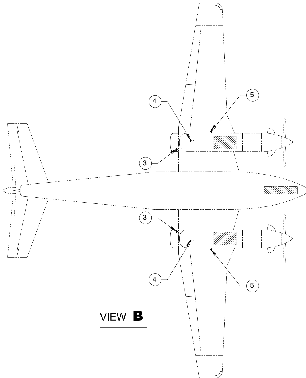
FIGURE 10-00 - PLACARDS, ST190 SHEET 2 OF 3
