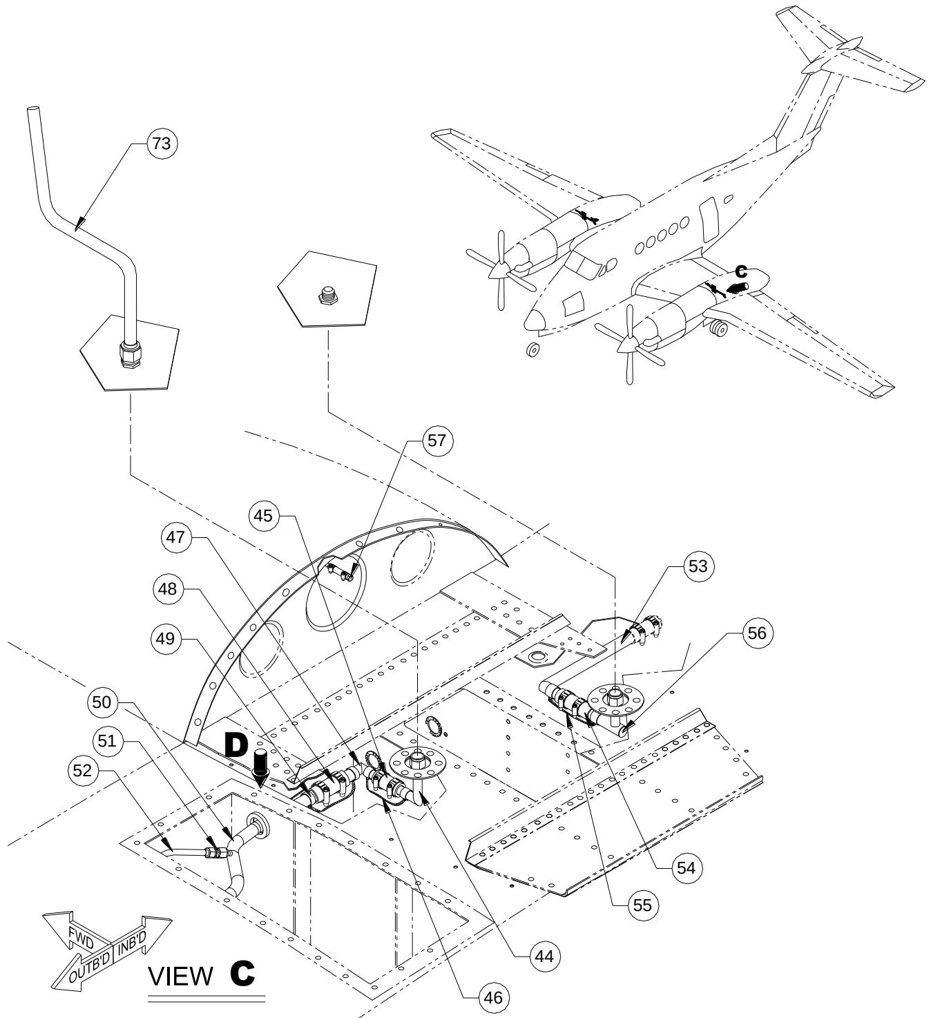
FIGURE 20-10 - FUEL SYSTEM INSTALLATION, ST190 SHEET 3 OF 4
