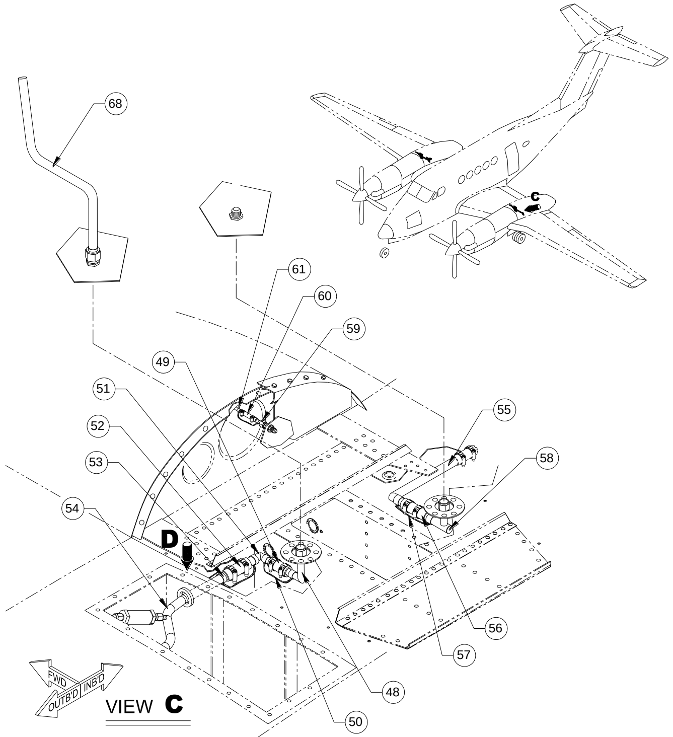
FIGURE 20-14 - FUEL SYSTEM INSTALLATION, ST120 (FM-3) SHEET 3 OF 4
