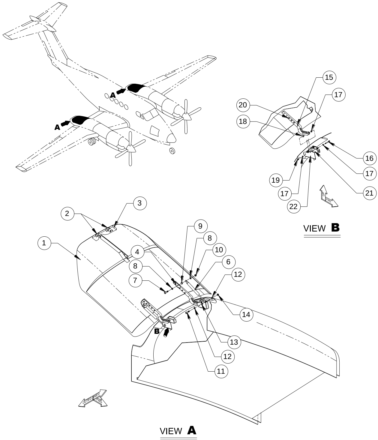
FIGURE 10-10 - SADDLE TANK STORAGE DOOR, ST120 SHEET 1 OF 2
