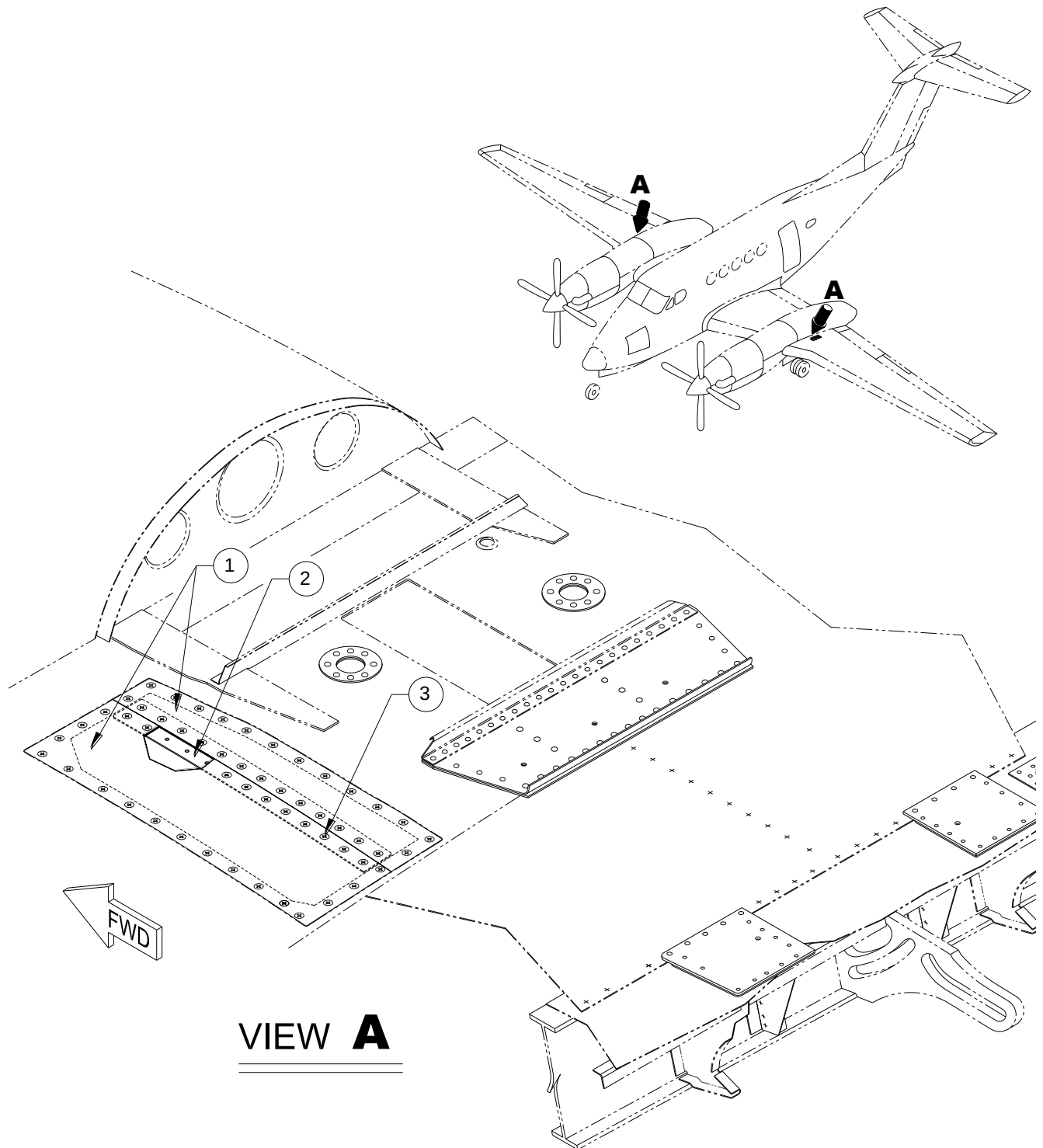
FIGURE 20-10 - MODIFIED INVERTER ACCESS PANEL DOOR
