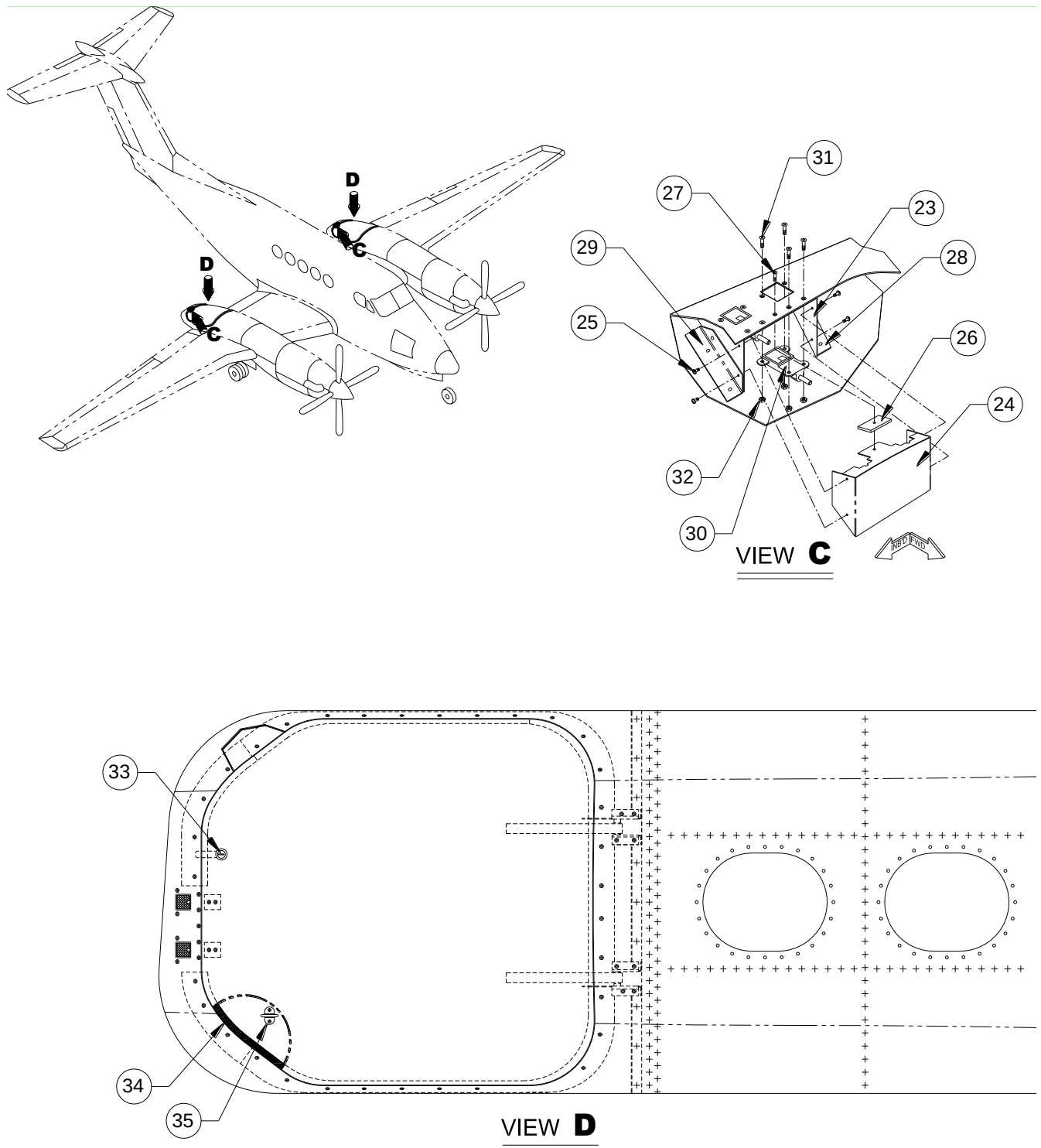
FIGURE 10-10 - SADDLE TANK STORAGE DOOR, ST120 SHEET 2 OF 2
