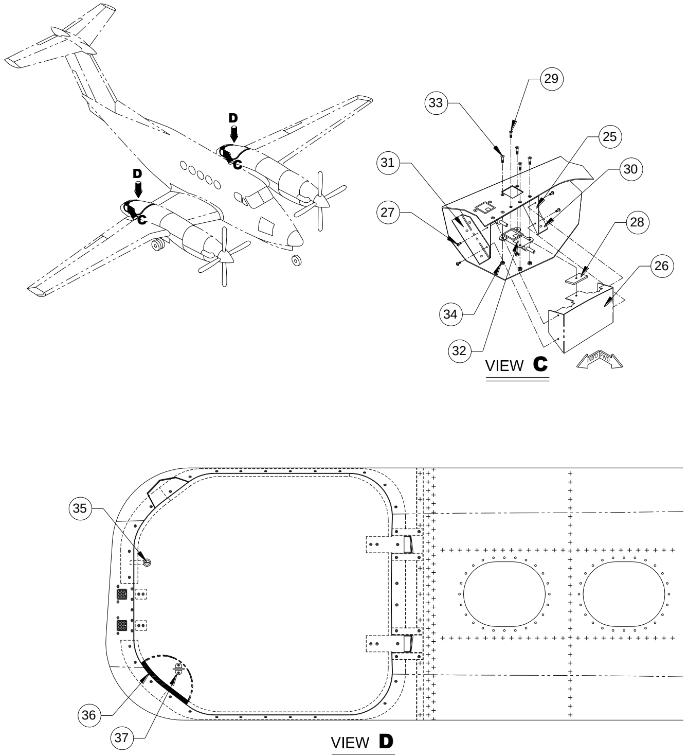
FIGURE 10-12 - SADDLE TANK STORAGE DOOR, ST120 (FM-3) SHEET 2 OF 2
