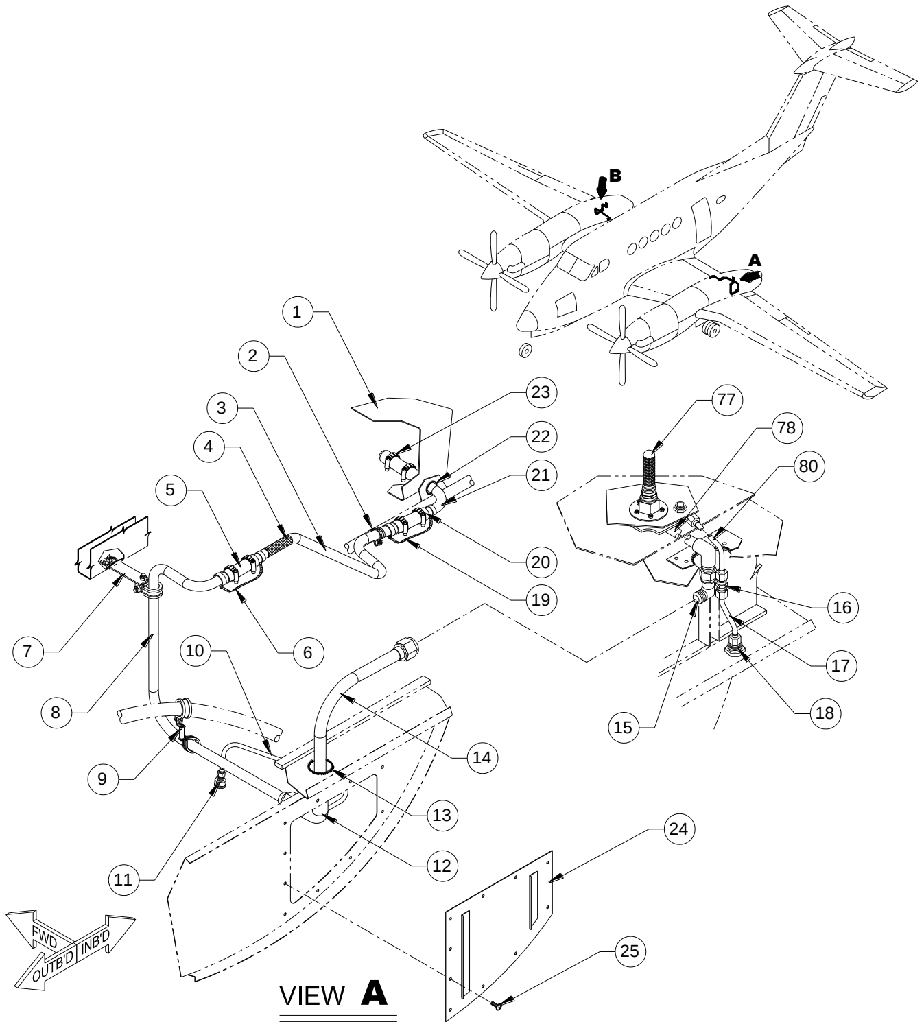
FIGURE 20-15 - FUEL SYSTEM INSTALLATION, ST72 SHEET 1 OF 4
