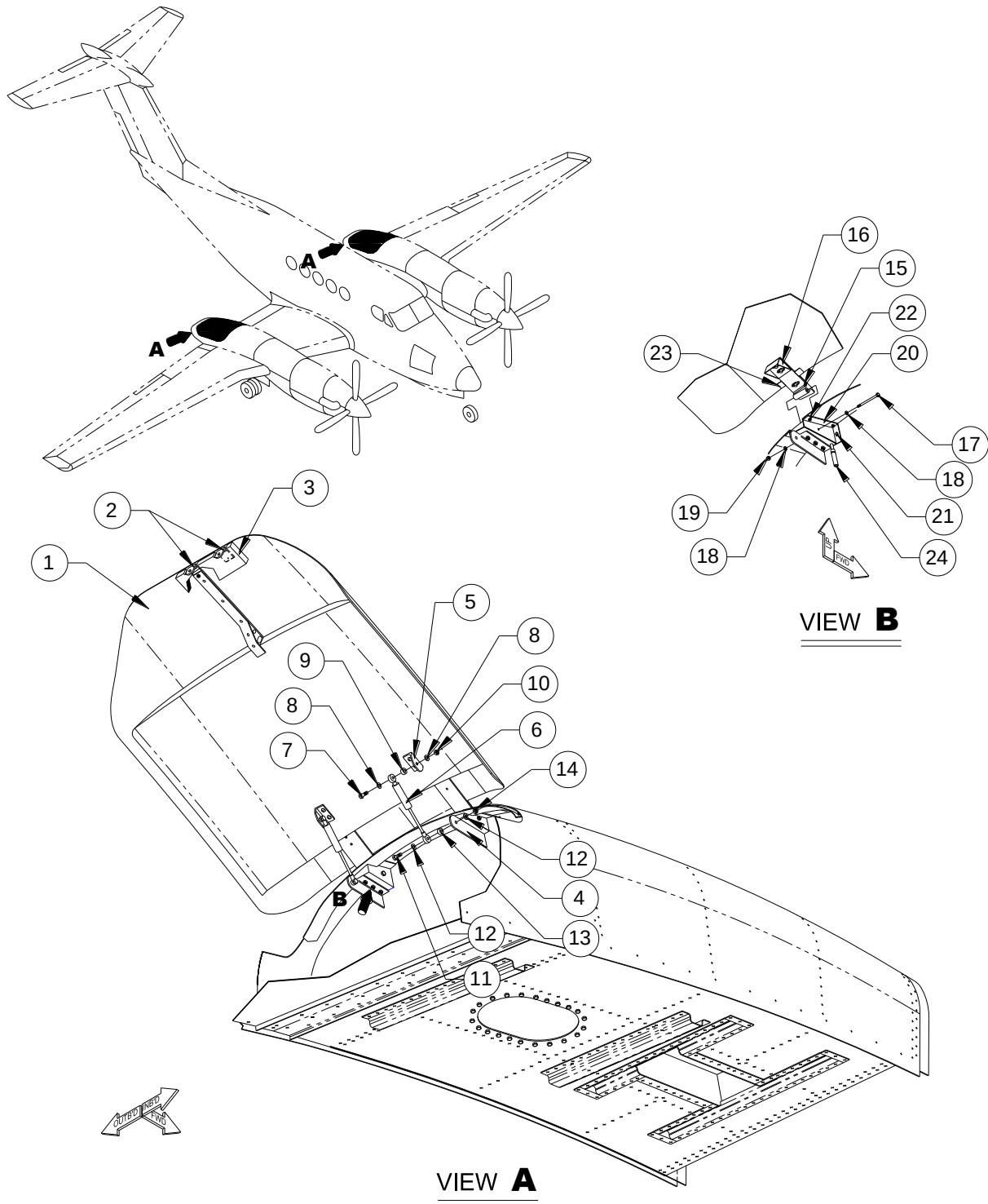
FIGURE 10-12 - SADDLE TANK STORAGE DOOR, ST120 (FM-3) SHEET 1 OF 2
