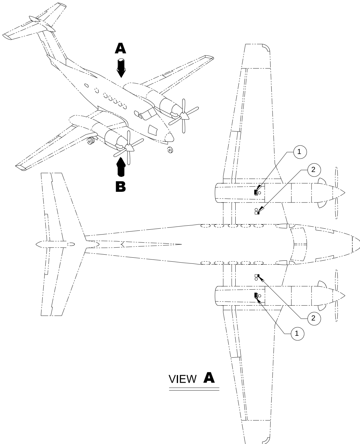
FIGURE 10-01 - PLACARDS, ST120 SHEET 1 OF 3
