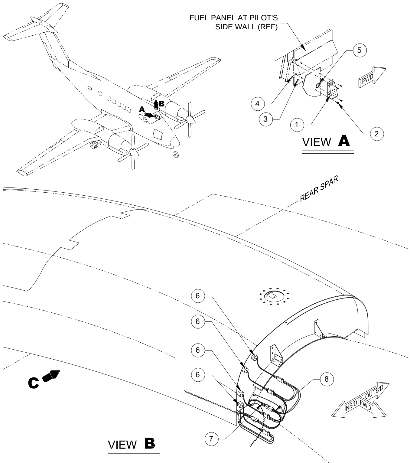
FIGURE 40-11 - FUEL LEVEL INDICATION, ST120 SHEET 1 OF 2
