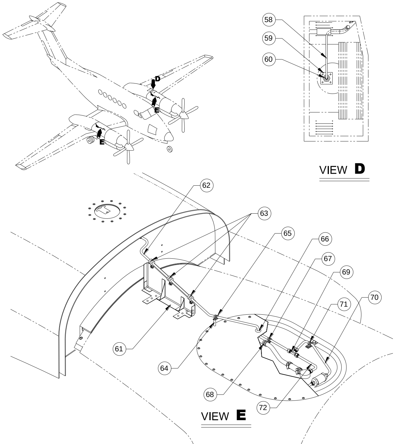
FIGURE 20-10 - FUEL SYSTEM INSTALLATION, ST190 SHEET 4 OF 4
