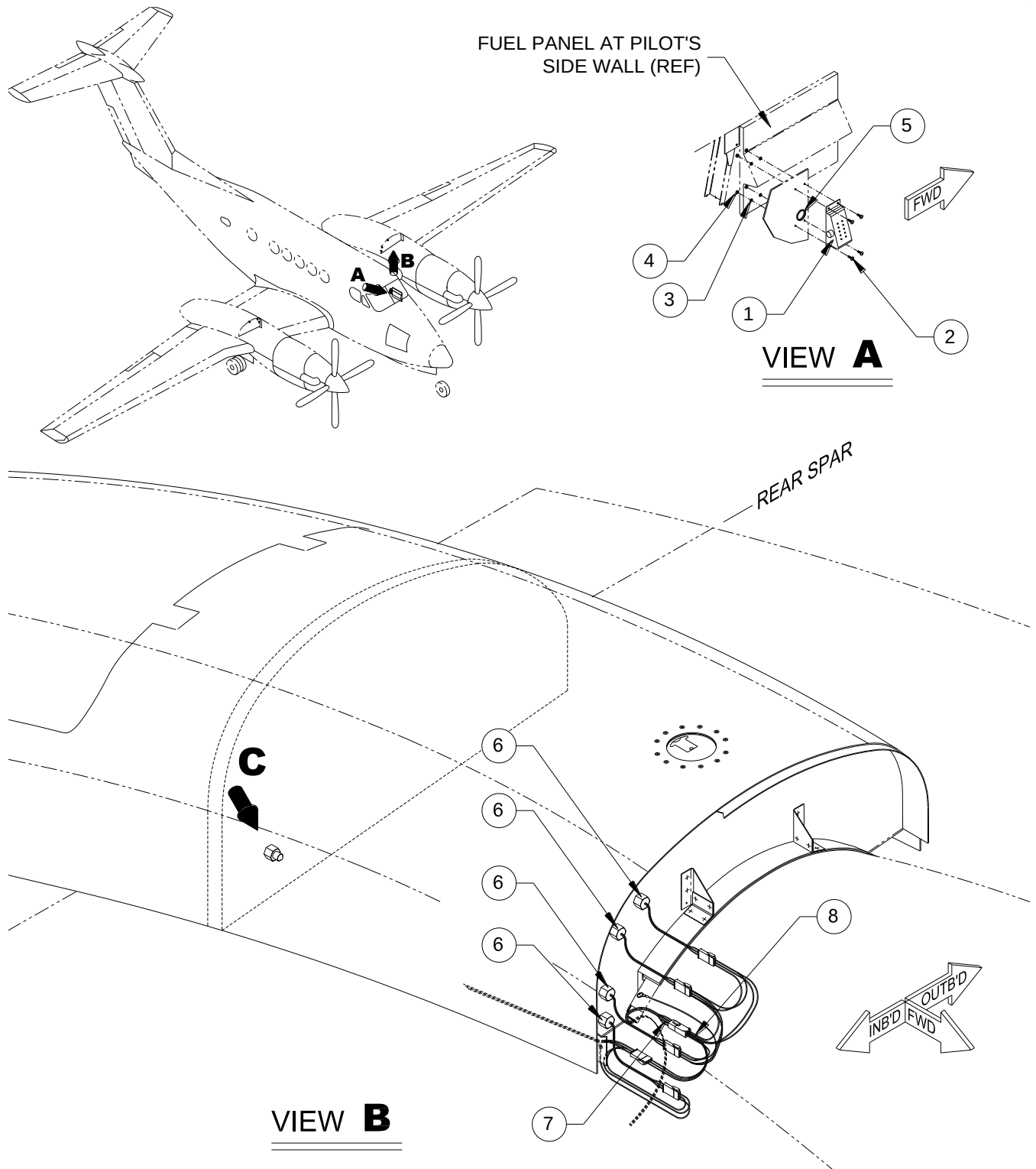
FIGURE 40-12 - FUEL LEVEL INDICATION, ST72 SHEET 1 OF 2
