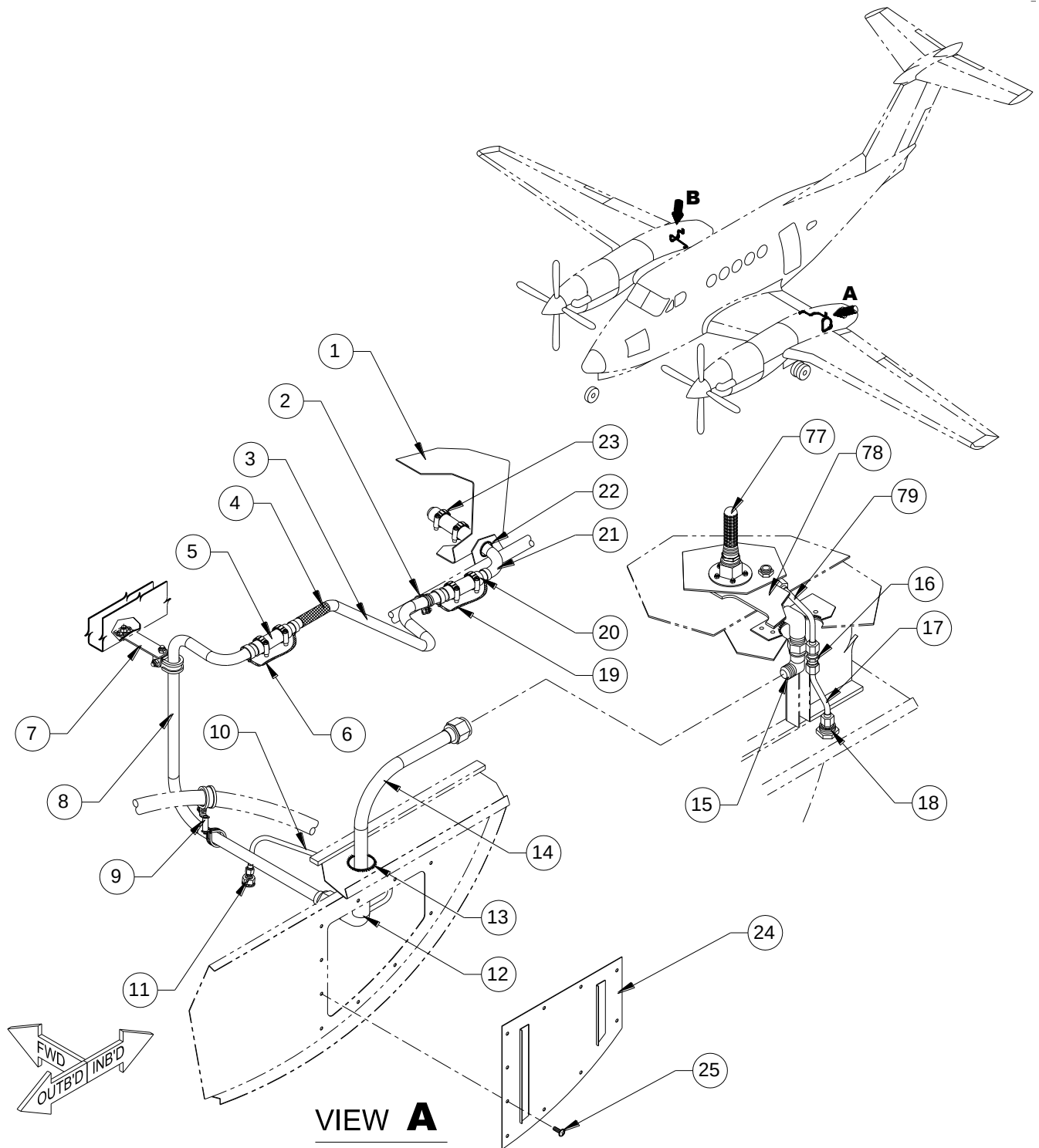
FIGURE 20-13 - FUEL SYSTEM INSTALLATION, ST120 SHEET 1 OF 4
