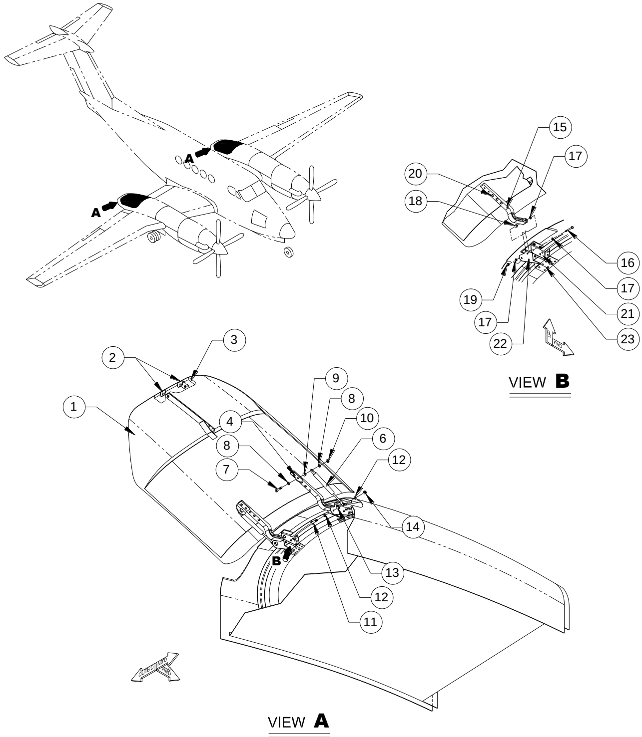
FIGURE 10-13 - SADDLE TANK STORAGE DOOR, ST72 SHEET 1 OF 2
