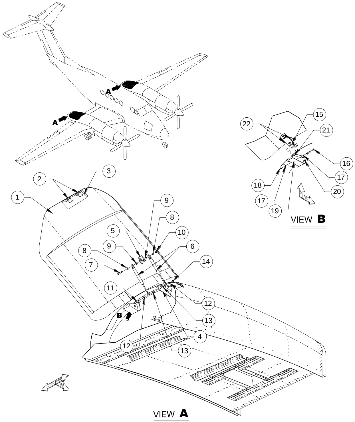
FIGURE 10-11 - SADDLE TANK STORAGE DOOR, ST120 (FL-360) SHEET 1 OF 2
