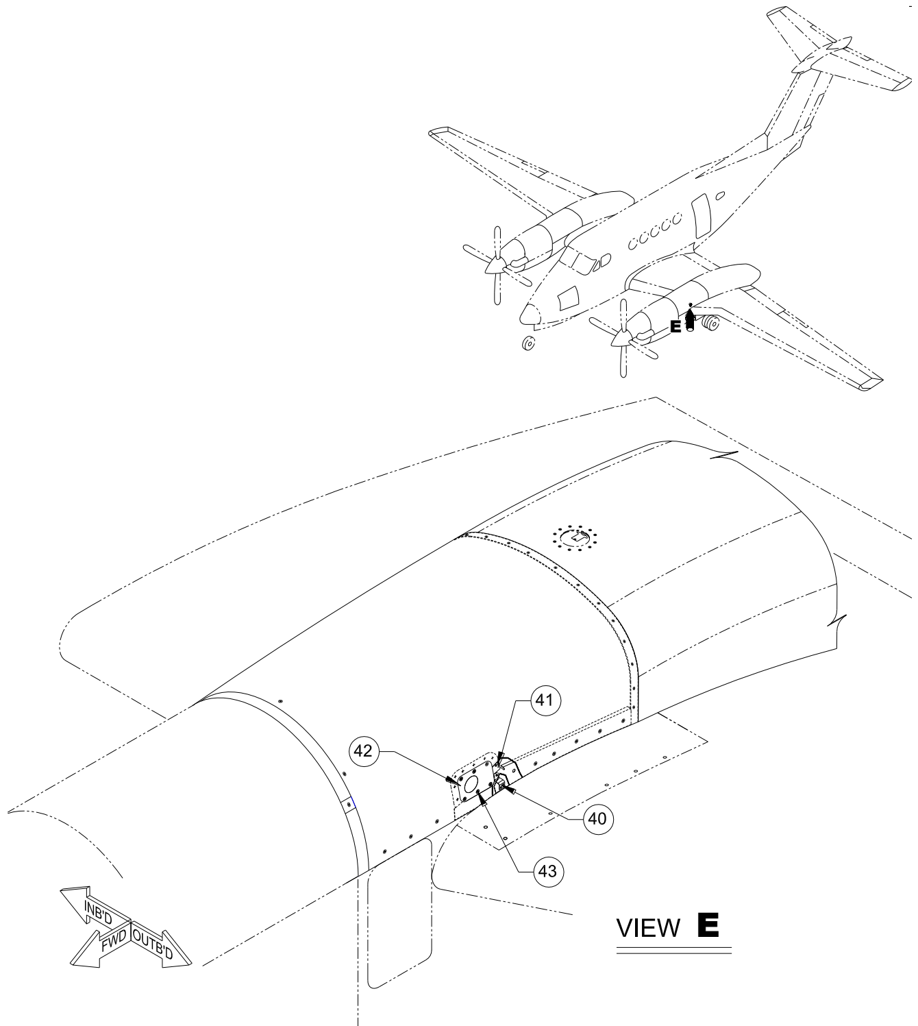
FIGURE 10-12 - SADDLE TANK FAIRINGS (300/B300) SHEET 3 OF 3
