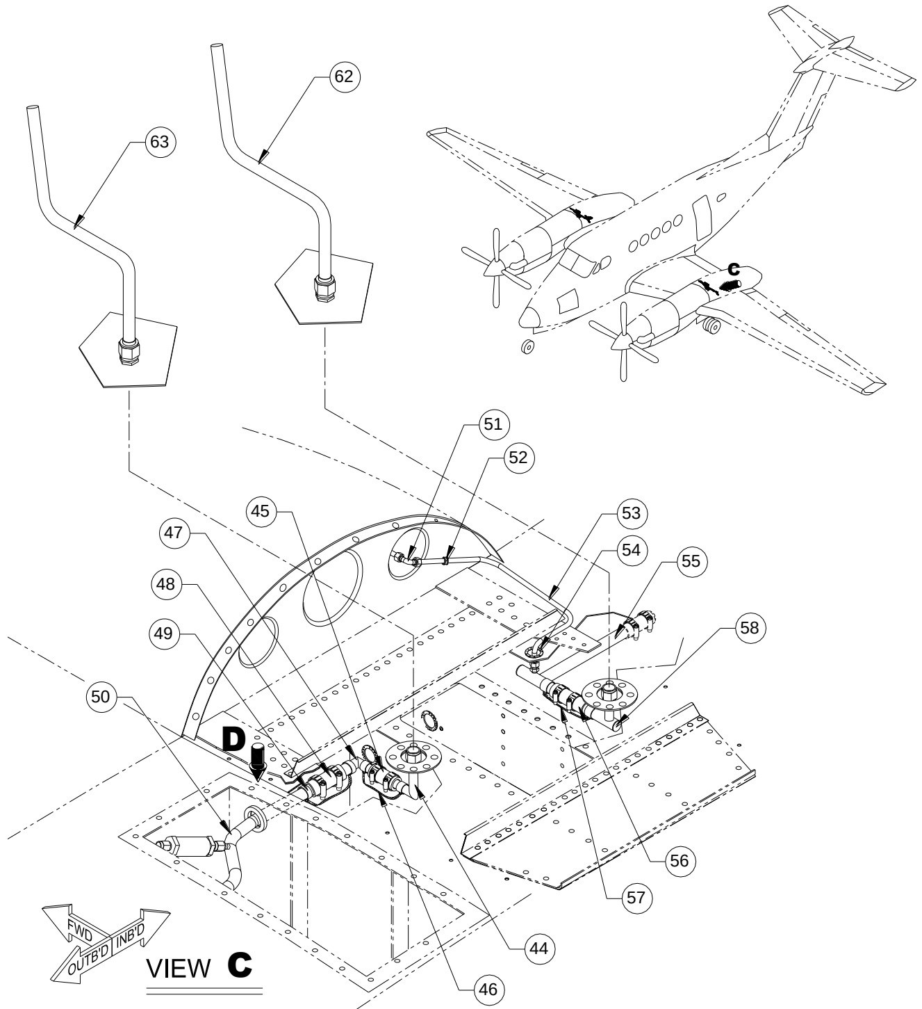
FIGURE 20-12 - FUEL SYSTEM INSTALLATION, ST190 (FL-31/-129/-241) SHEET 3 OF 4
