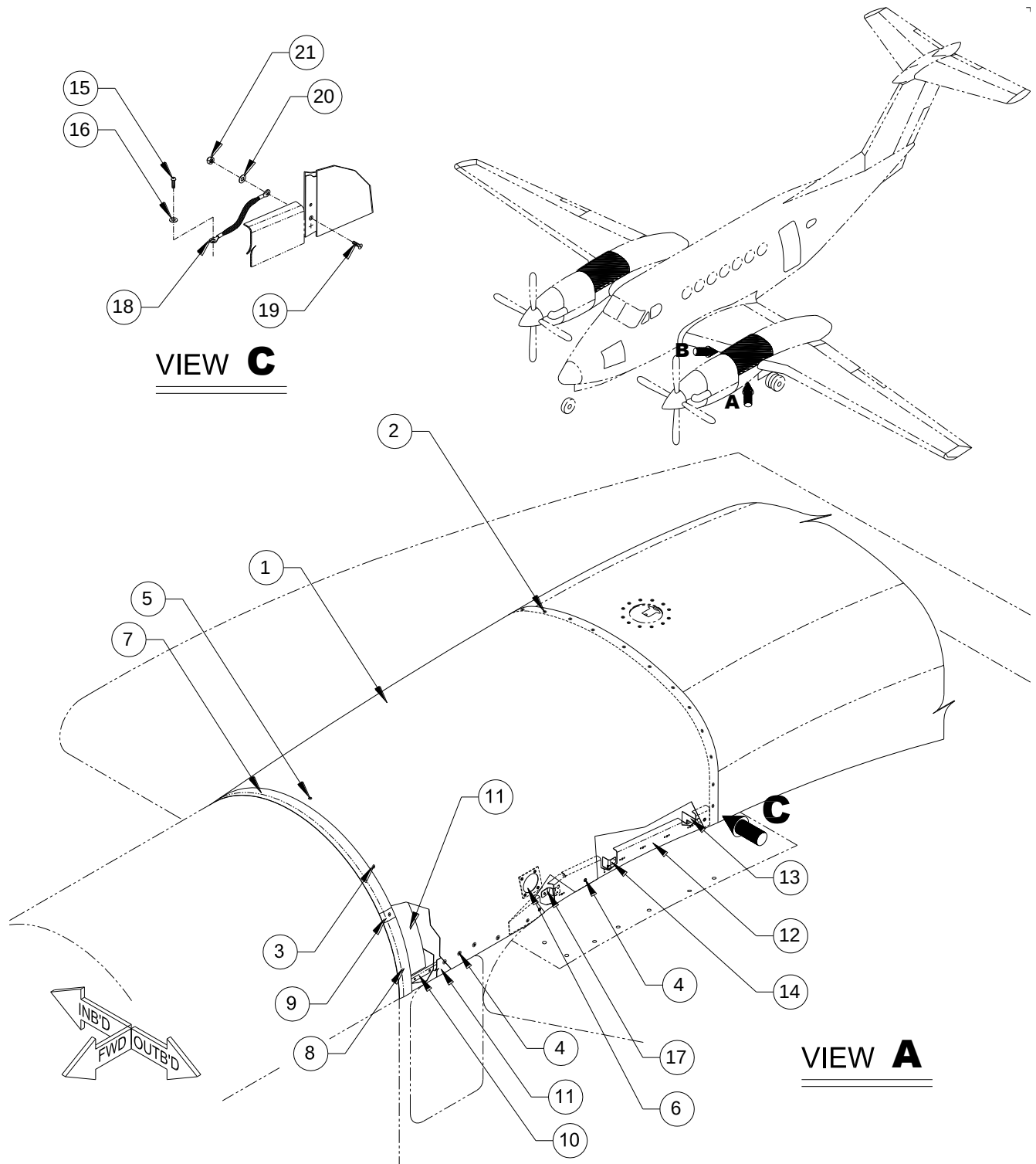
FIGURE 10-12 - SADDLE TANK FAIRINGS (300/B300) SHEET 1 OF 3
