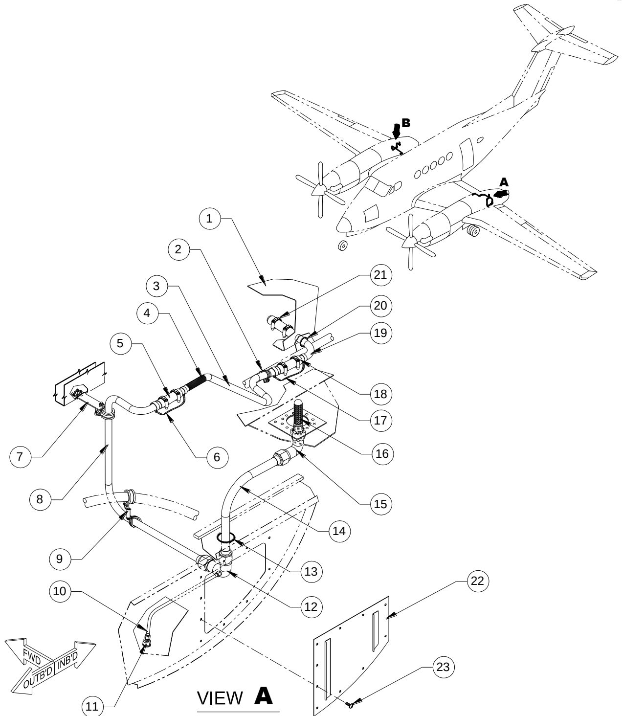
FIGURE 20-11 - FUEL SYSTEM INSTALLATION, ST190 (BL-7) SHEET 1 OF 4
