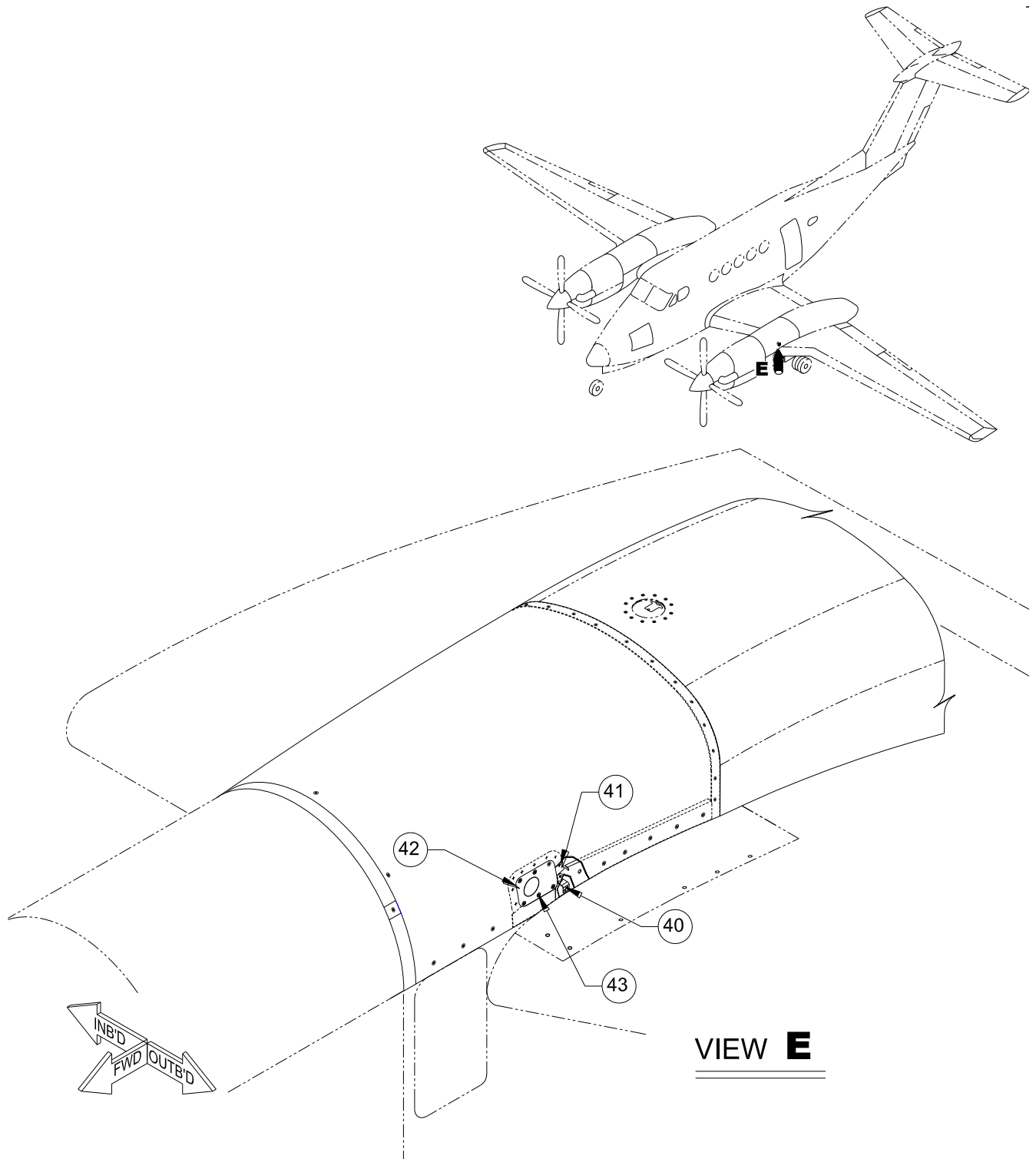
FIGURE 10-10 - SADDLE TANK FAIRINGS (200/B200) SHEET 3 OF 3
