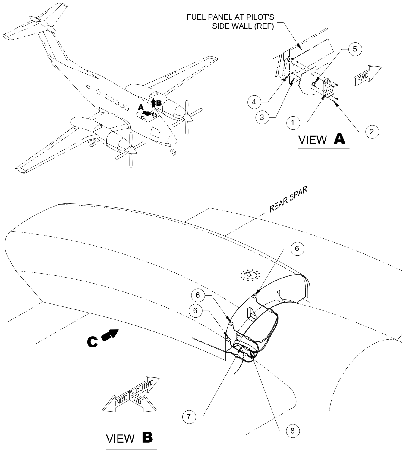
FIGURE 40-10 - FUEL LEVEL INDICATION, ST190 SHEET 1 OF 2
