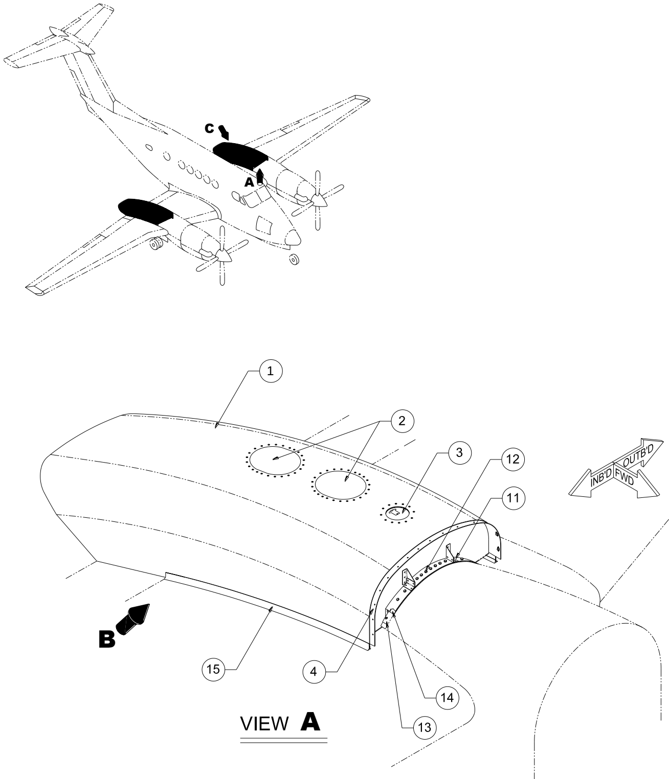
FIGURE 10-10 - SADDLE TANKS INSTALLATION, ST190 SHEET 1 OF 4
