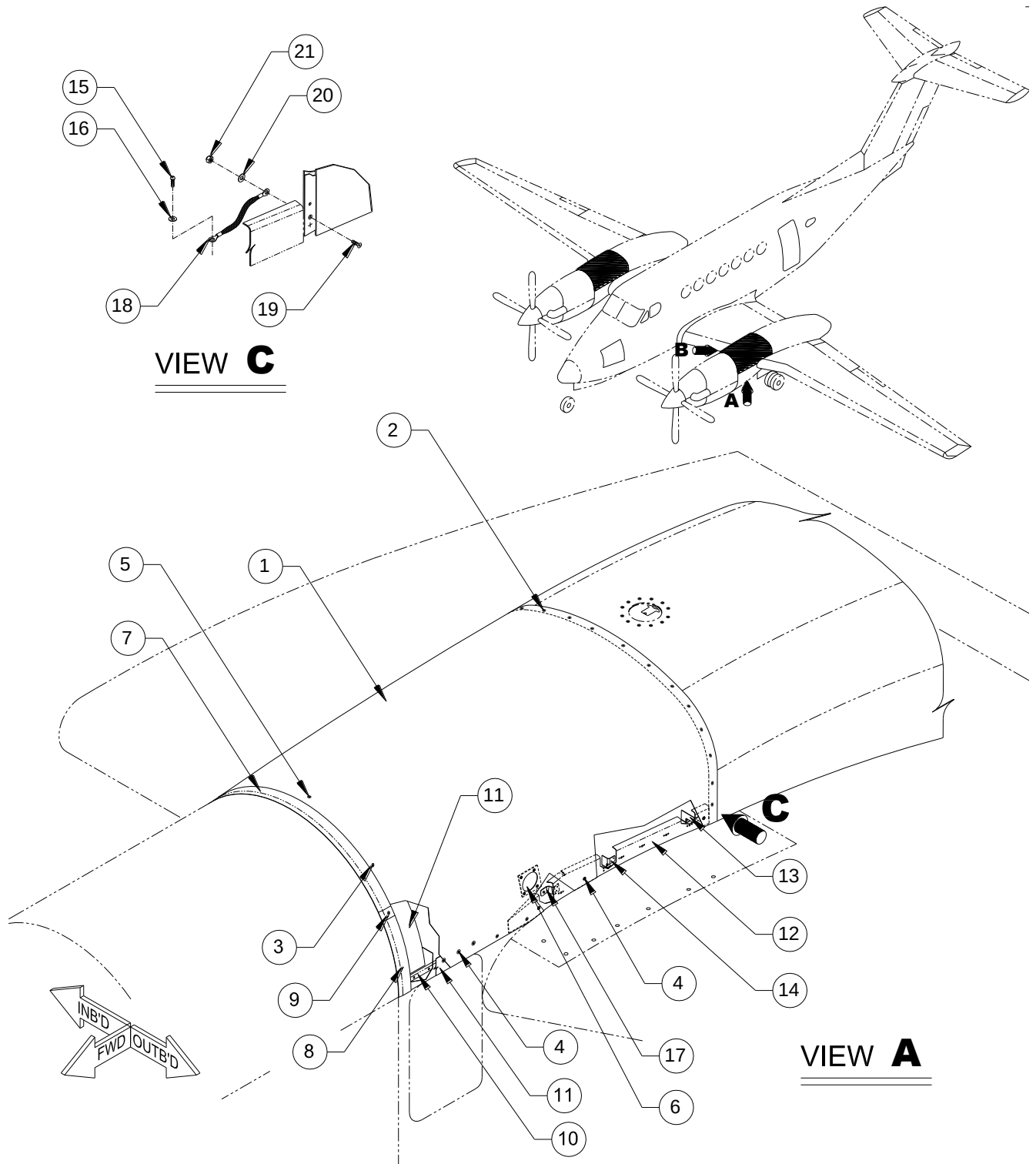
FIGURE 10-10 - SADDLE TANK FAIRINGS (200/B200) SHEET 1 OF 3
