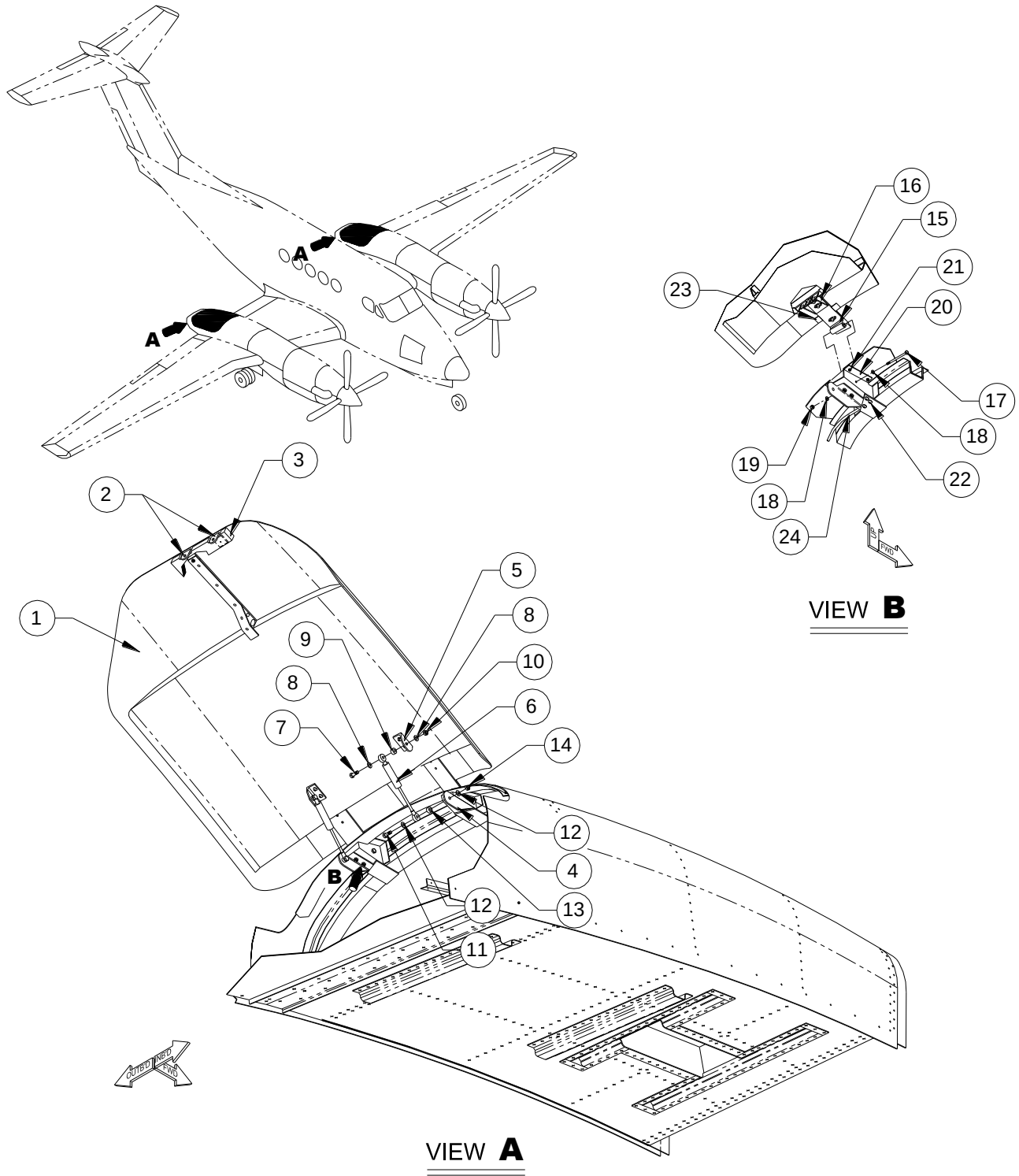
FIGURE 10-15 - SADDLE TANK STORAGE DOOR, ST72 (BL-46) SHEET 1 OF 2
