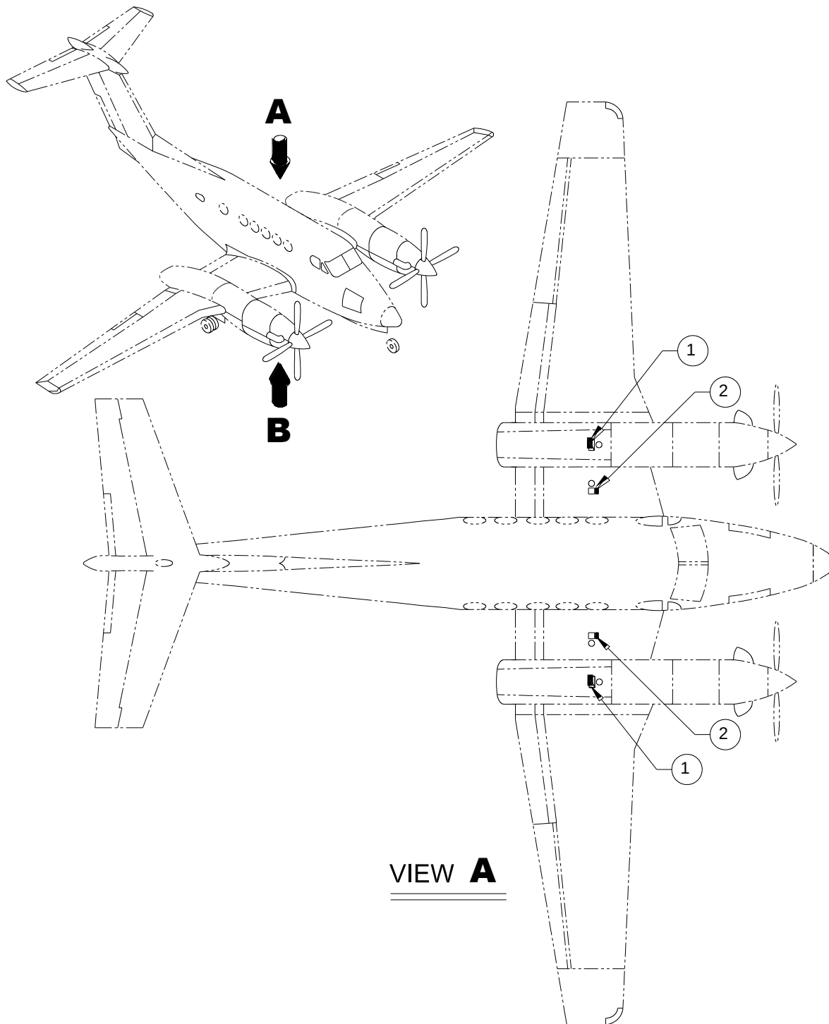
FIGURE 10-00 - PLACARDS, ST190 SHEET 1 OF 3
