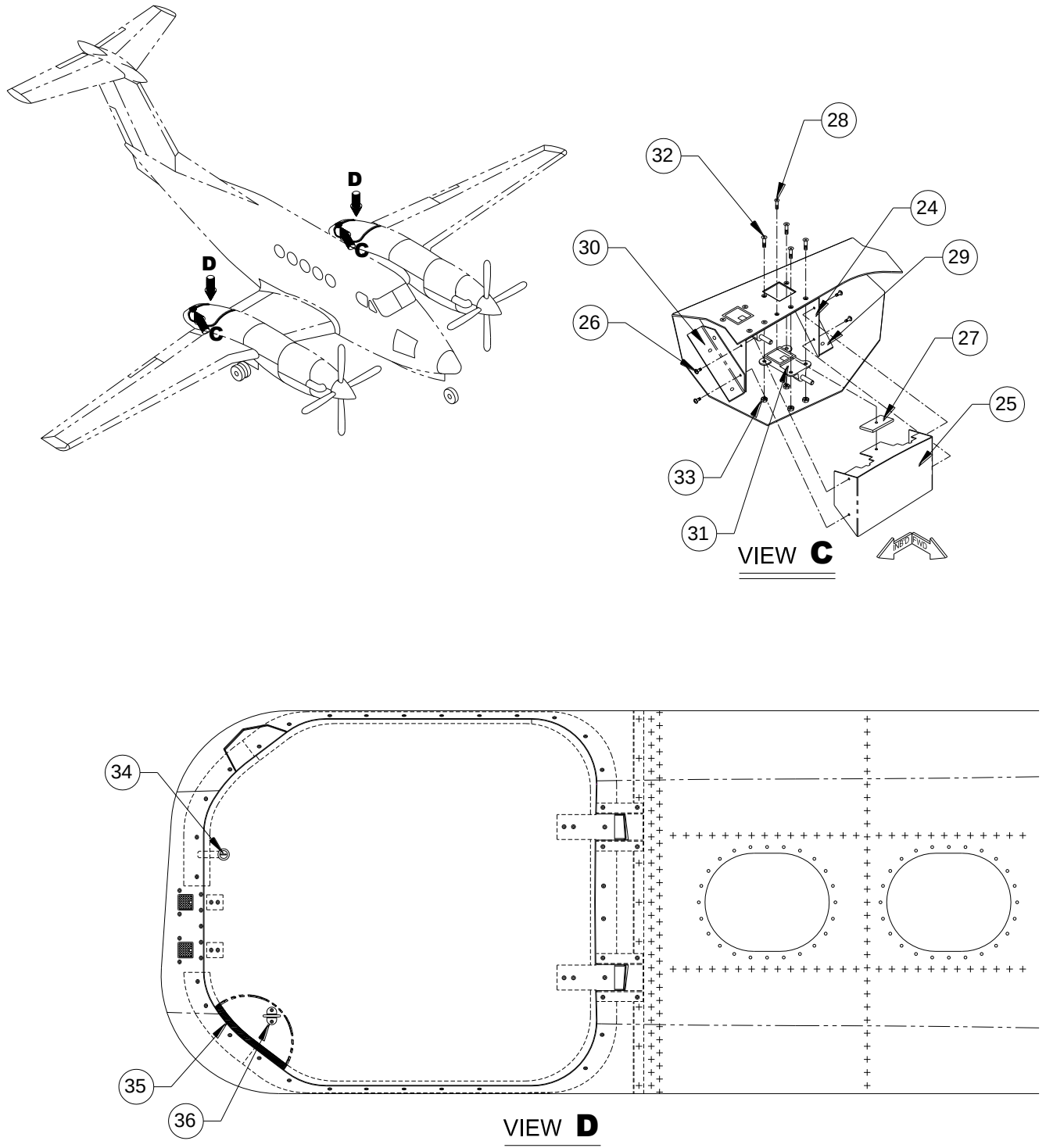
FIGURE 10-11 - SADDLE TANK STORAGE DOOR, ST120 (FL-360) SHEET 2 OF 2
