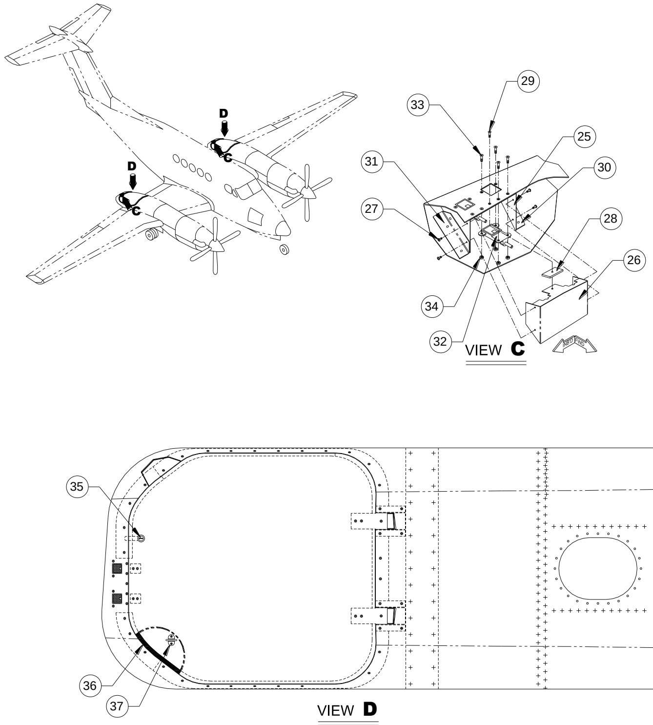
FIGURE 10-15 - SADDLE TANK STORAGE DOOR, ST72 (BL-46) SHEET 2 OF 2
