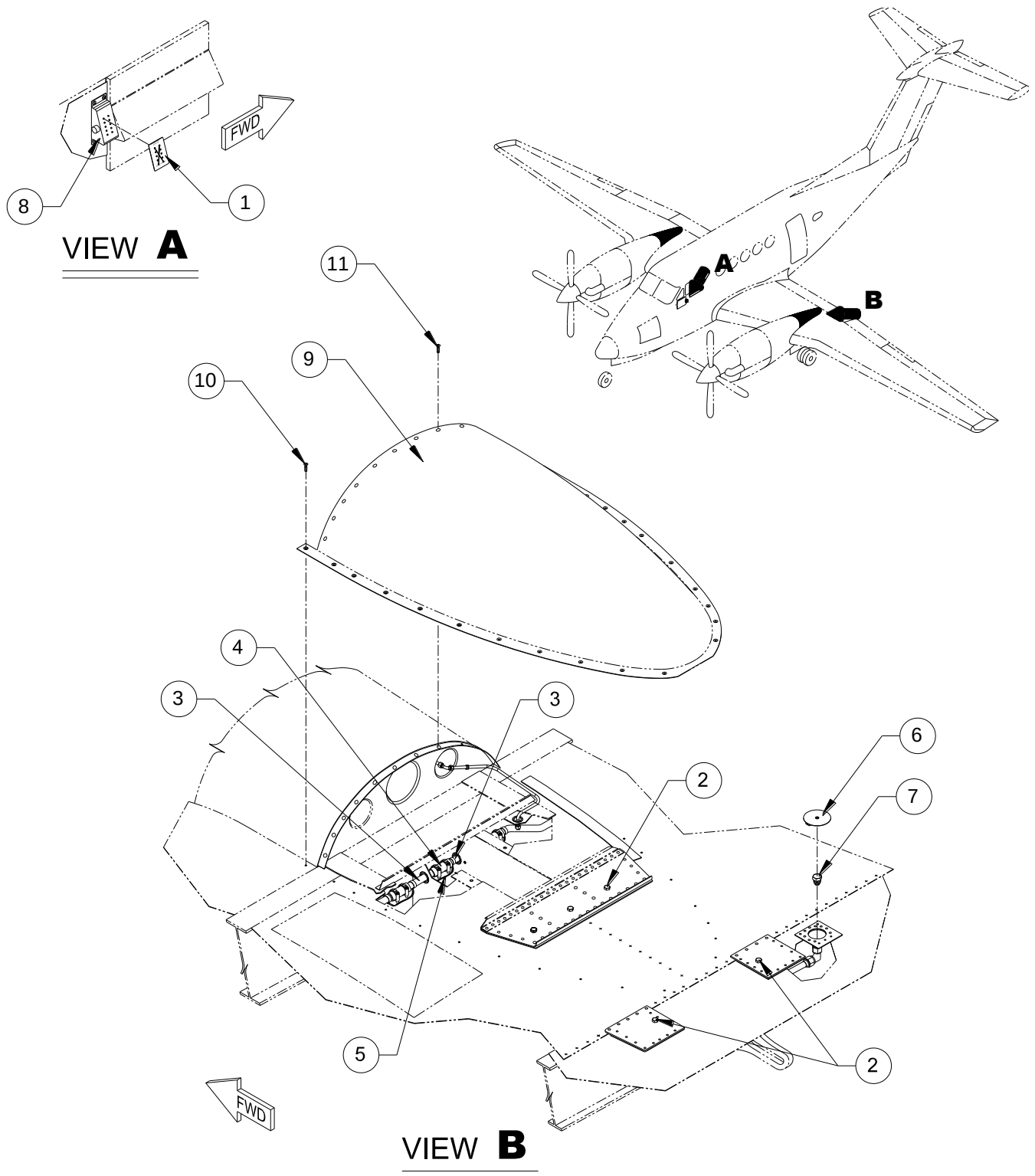
FIGURE 15-12 - SADDLE TANKS REMOVED CONFIGURATION (S/N BL-7)
