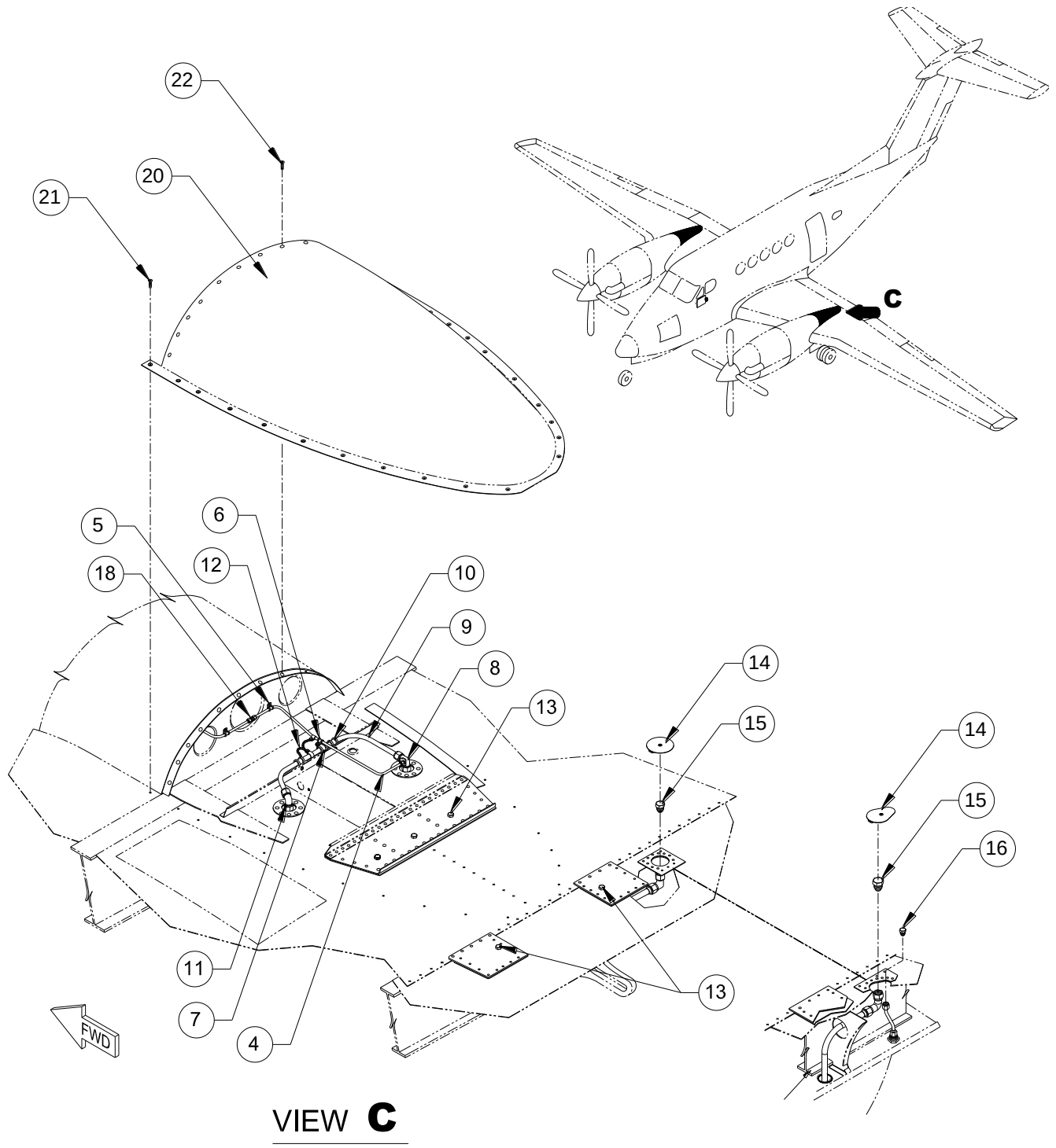
FIGURE 15-10 - SADDLE TANKS REMOVED CONFIGURATION (REVISED) SHEET 2 OF 2
