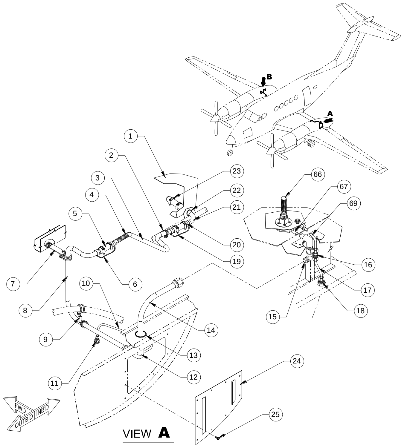
FIGURE 20-16 - FUEL SYSTEM INSTALLATION, ST72 (BB-1239) SHEET 1 OF 4
