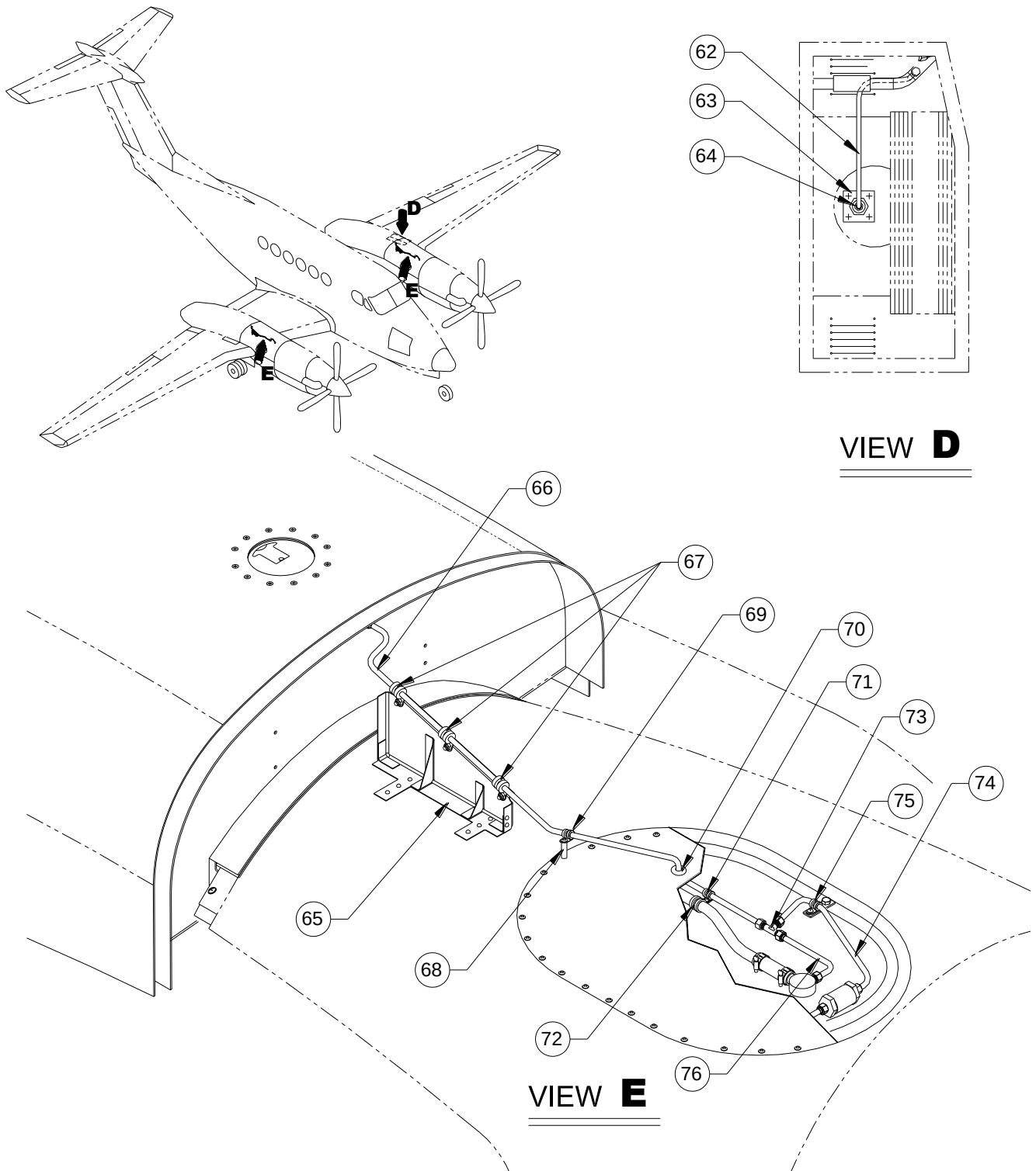
FIGURE 20-13 - FUEL SYSTEM INSTALLATION, ST120 SHEET 4 OF 4
