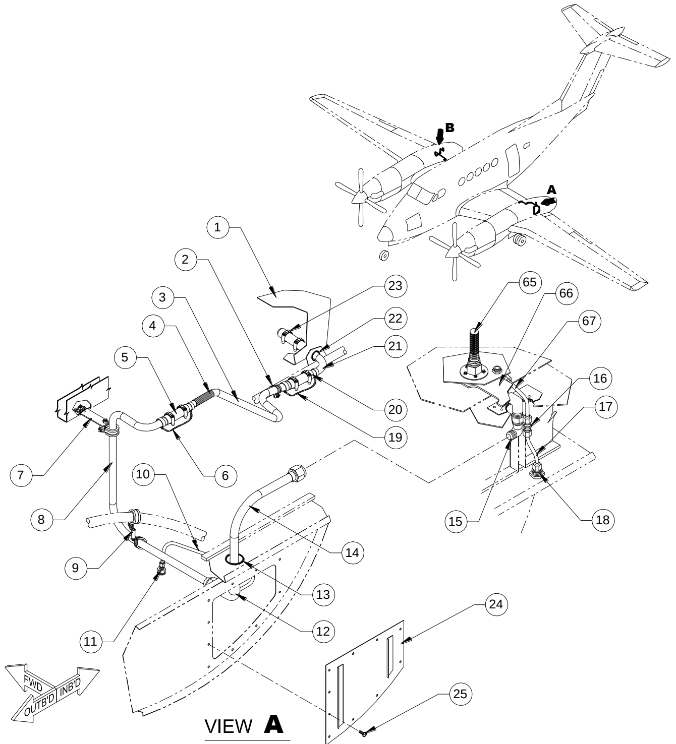
FIGURE 20-14 - FUEL SYSTEM INSTALLATION, ST120 (FM-3) SHEET 1 OF 4
