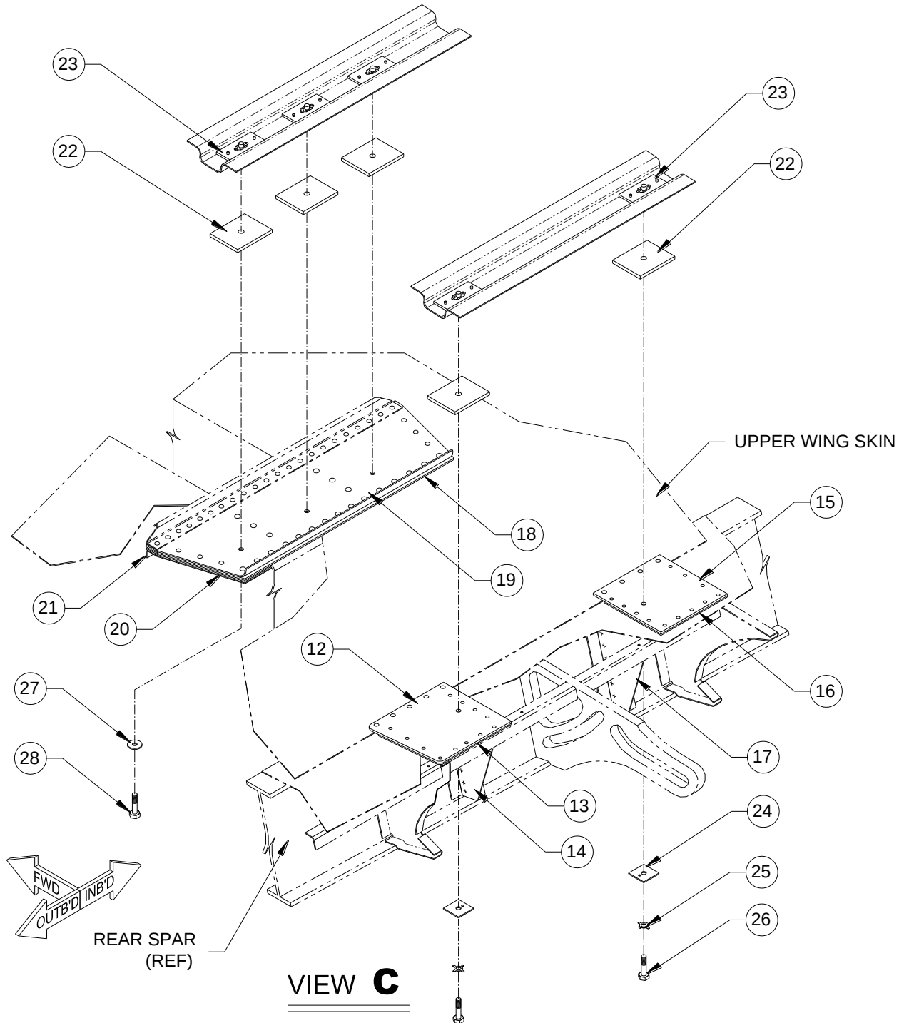
FIGURE 10-11 - SADDLE TANKS INSTALLATION, ST120/ST72 SHEET 3 OF 4
