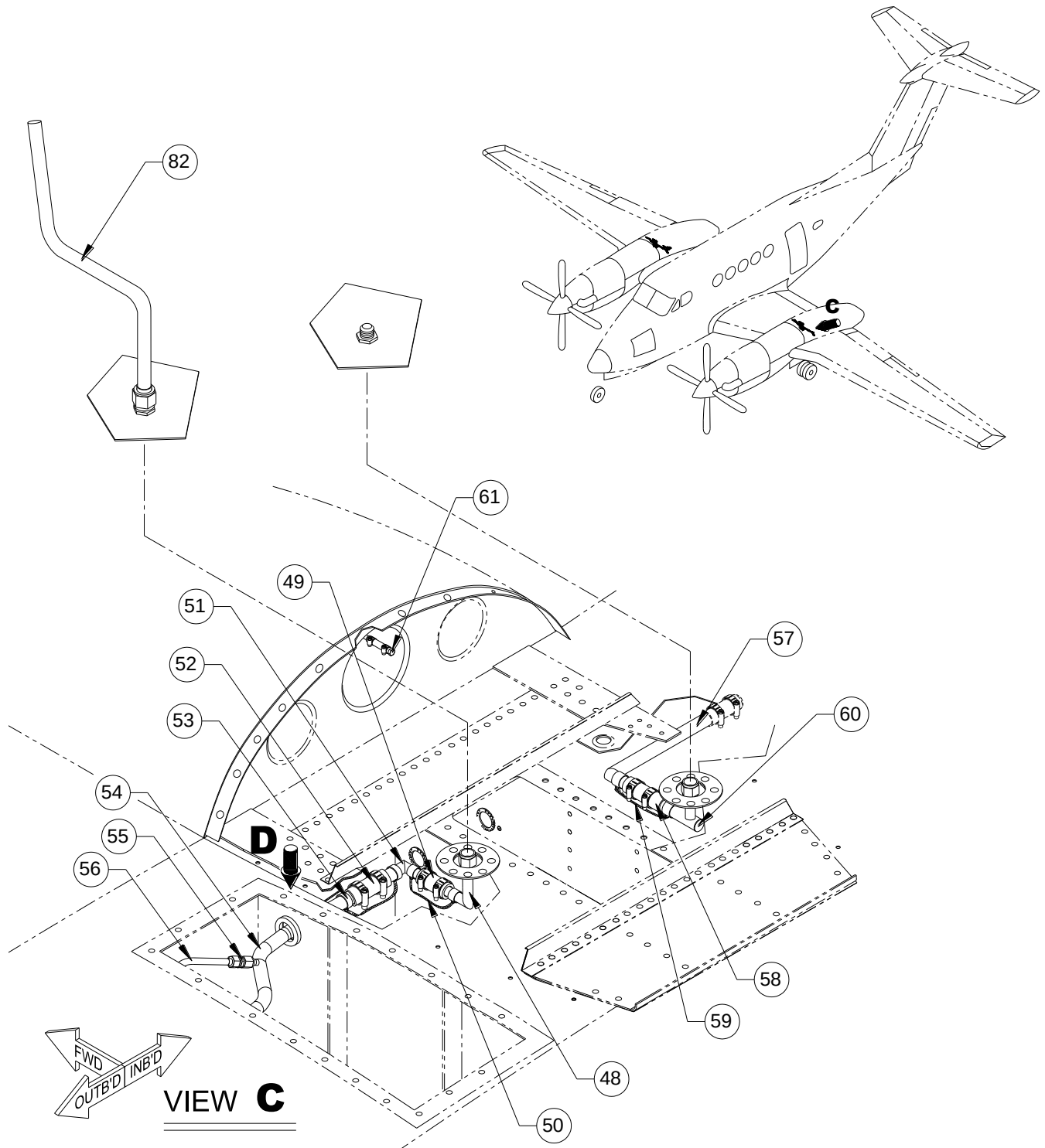
FIGURE 20-15 - FUEL SYSTEM INSTALLATION, ST72 SHEET 3 OF 4
