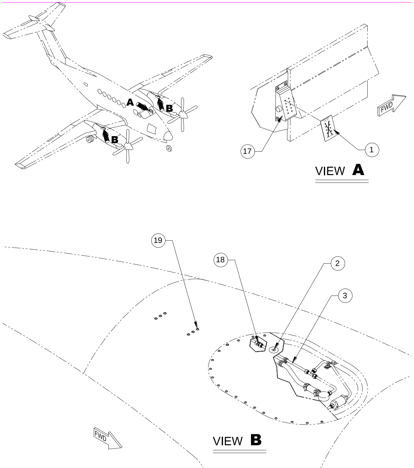
FIGURE 15-10 - SADDLE TANKS REMOVED CONFIGURATION (REVISED) SHEET 1 OF 2
