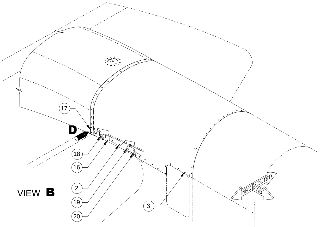
FIGURE 10-11 - SADDLE TANK FAIRINGS (BL-7) SHEET 2 OF 2
