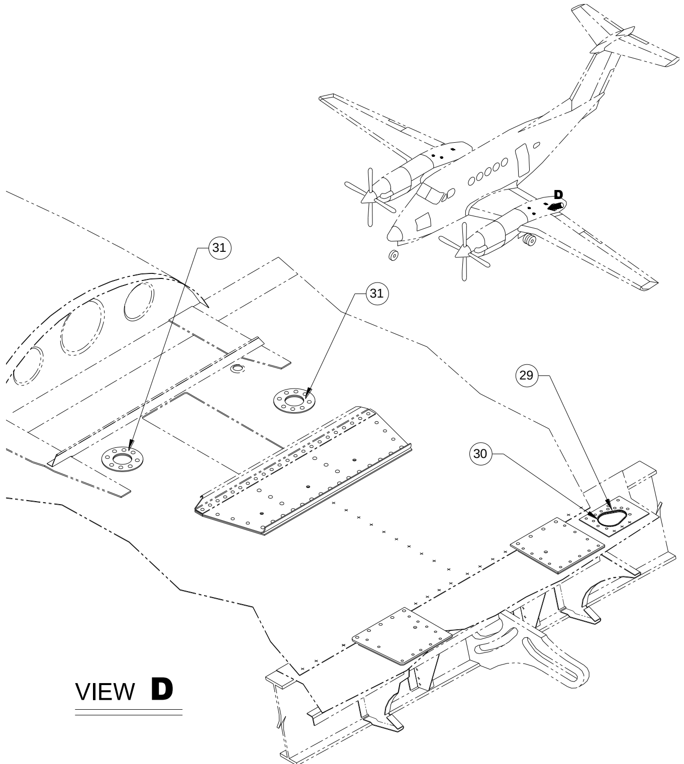
FIGURE 10-11 - SADDLE TANKS INSTALLATION, ST120/ST72 SHEET 4 OF 4
