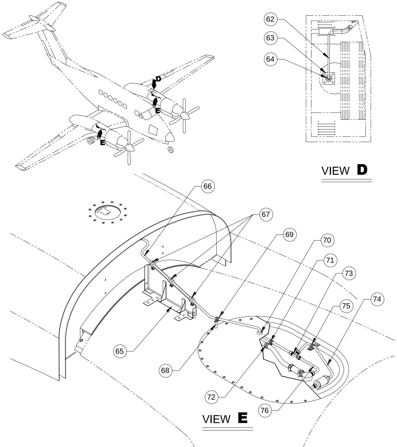
FIGURE 20-15 - FUEL SYSTEM INSTALLATION, ST72 SHEET 4 OF 4
