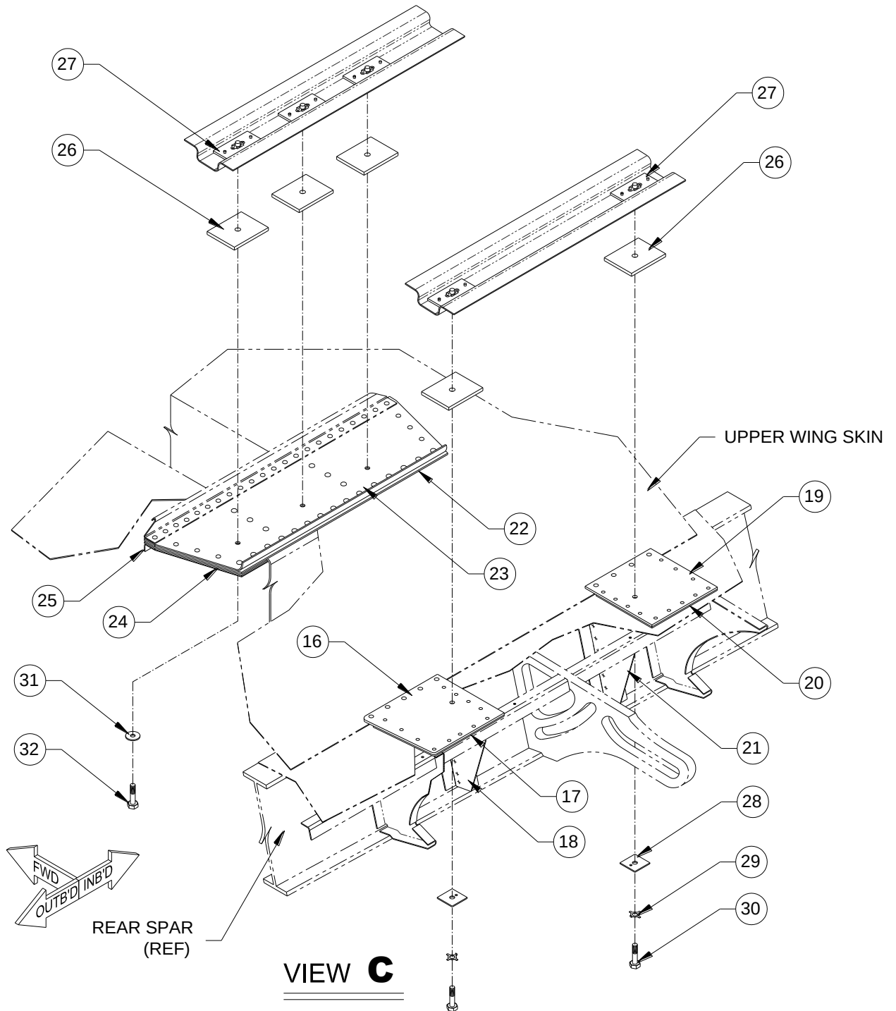
FIGURE 10-10 - SADDLE TANKS INSTALLATION, ST190 SHEET 3 OF 4
