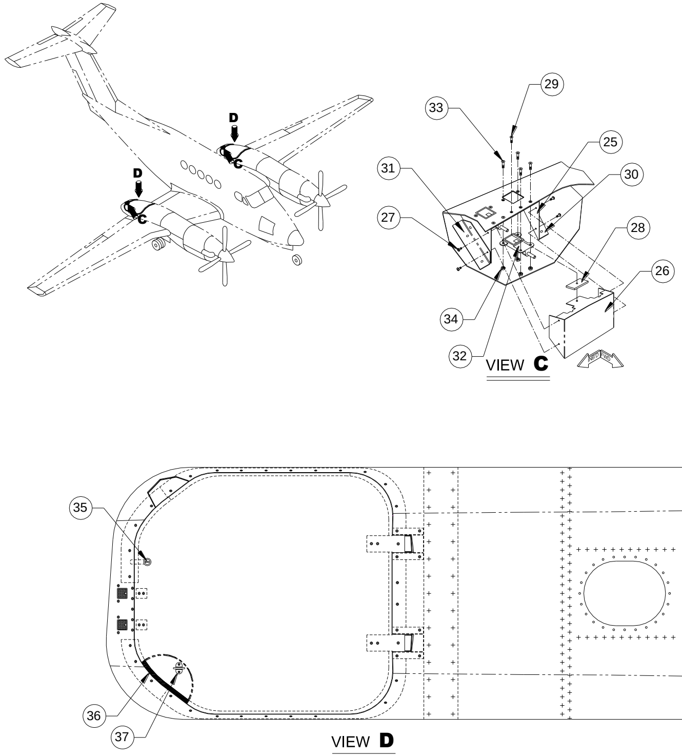
FIGURE 10-14 - SADDLE TANK STORAGE DOOR, ST72 (BB-1239) SHEET 2 OF 2
