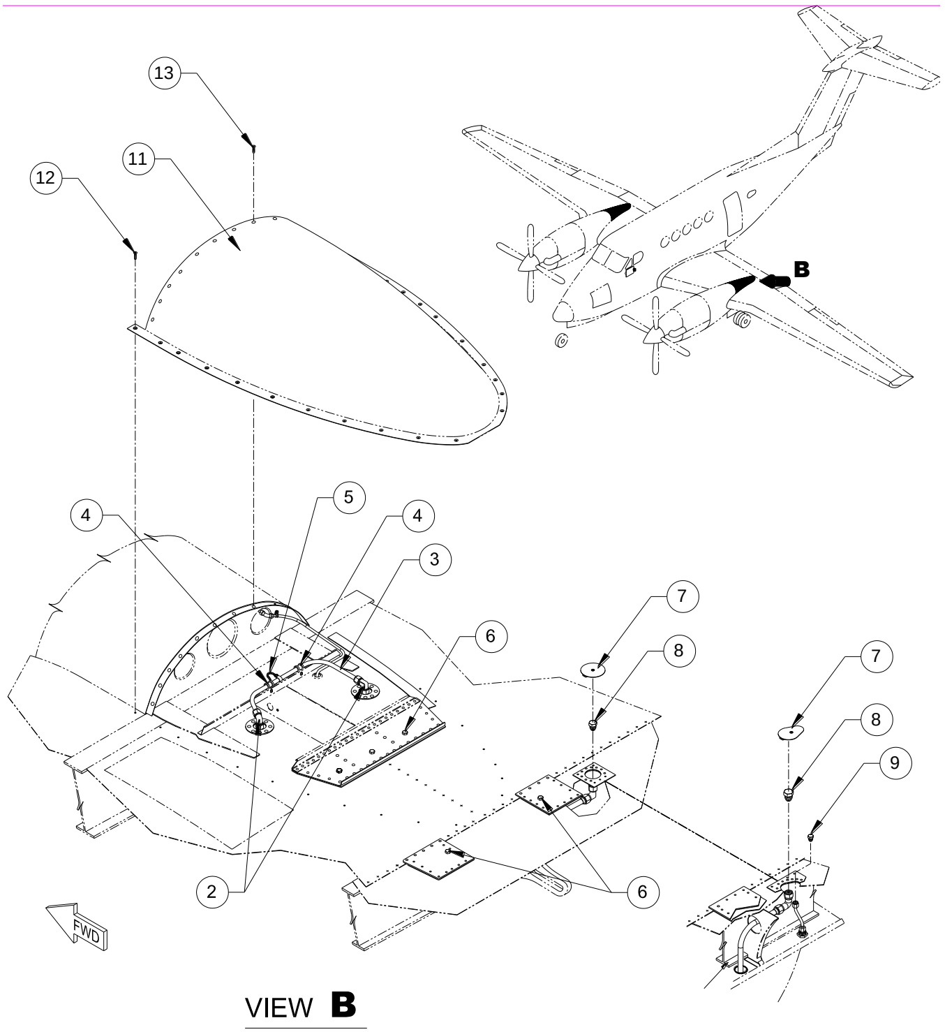
FIGURE 15-11 - SADDLE TANKS REMOVED CONFIGURATION (ORIGINAL) SHEET 2 OF 2
