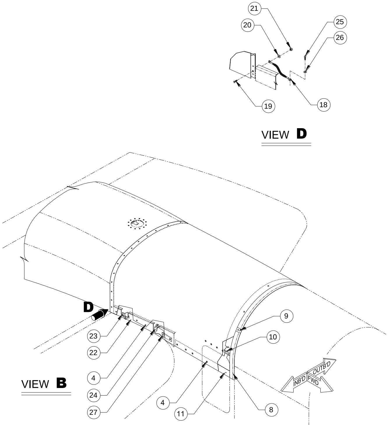
FIGURE 10-10 - SADDLE TANK FAIRINGS (200/B200) SHEET 2 OF 3
