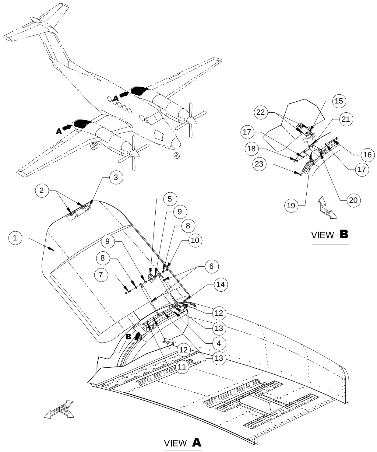
FIGURE 10-14 - SADDLE TANK STORAGE DOOR, ST72 (BB-1239) SHEET 1 OF 2
