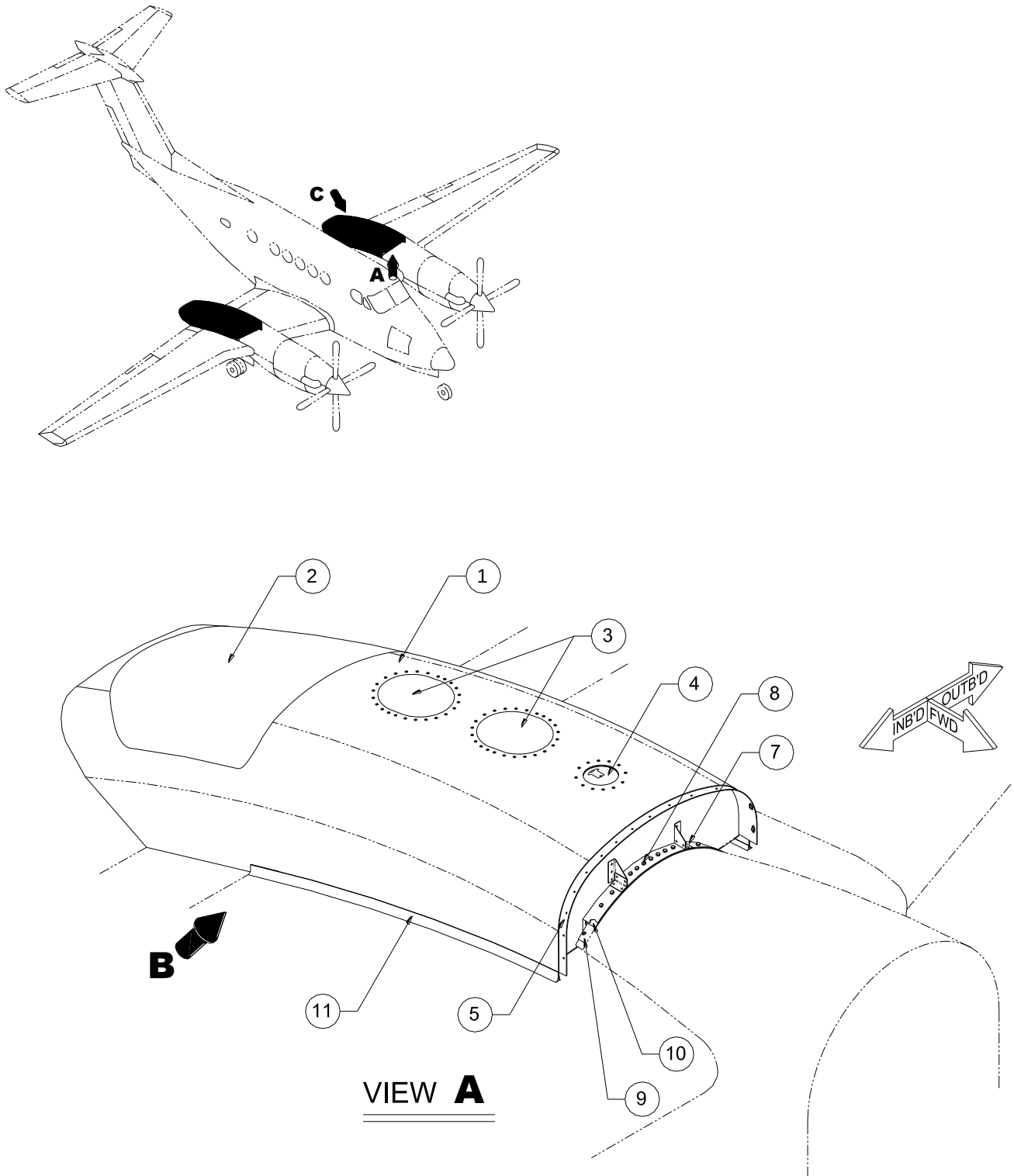
FIGURE 10-11 - SADDLE TANKS INSTALLATION, ST120/ST72 SHEET 1 OF 4
