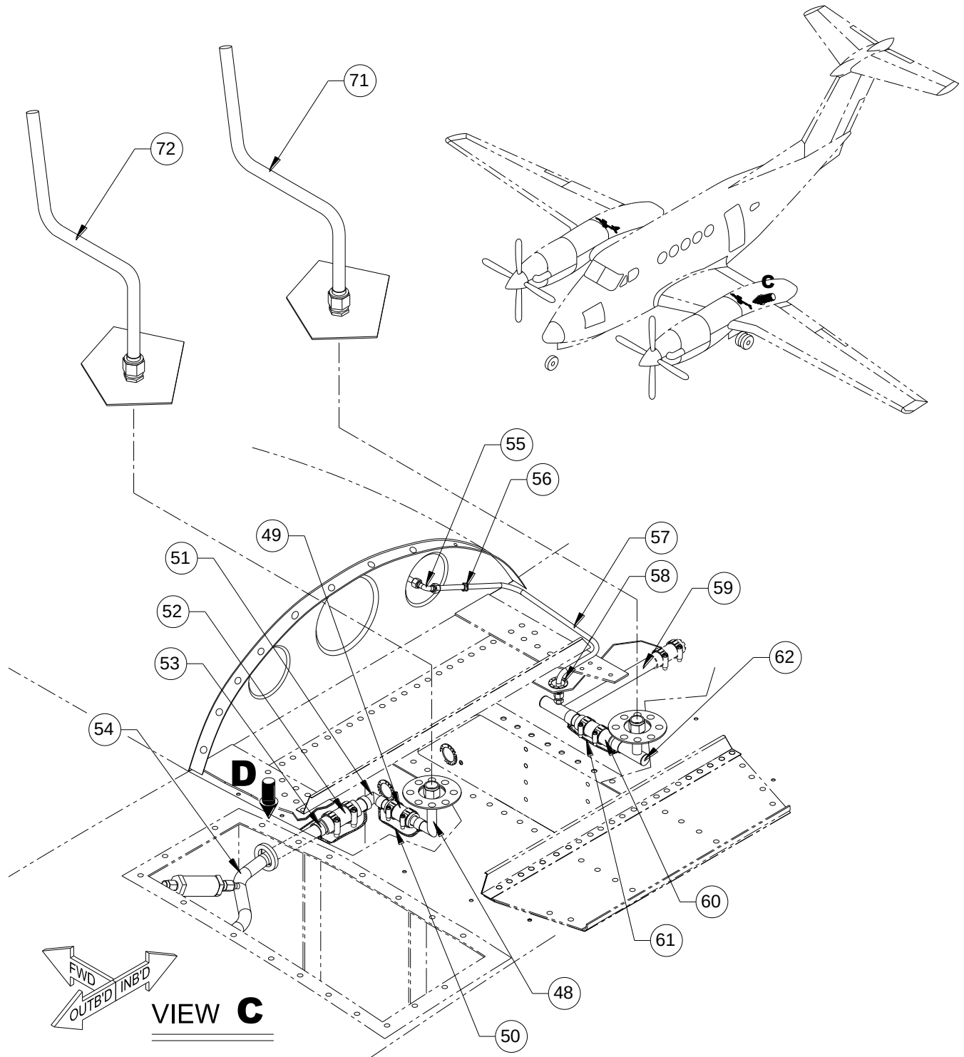
FIGURE 20-16 - FUEL SYSTEM INSTALLATION, ST72 (BB-1239) SHEET 3 OF 4
