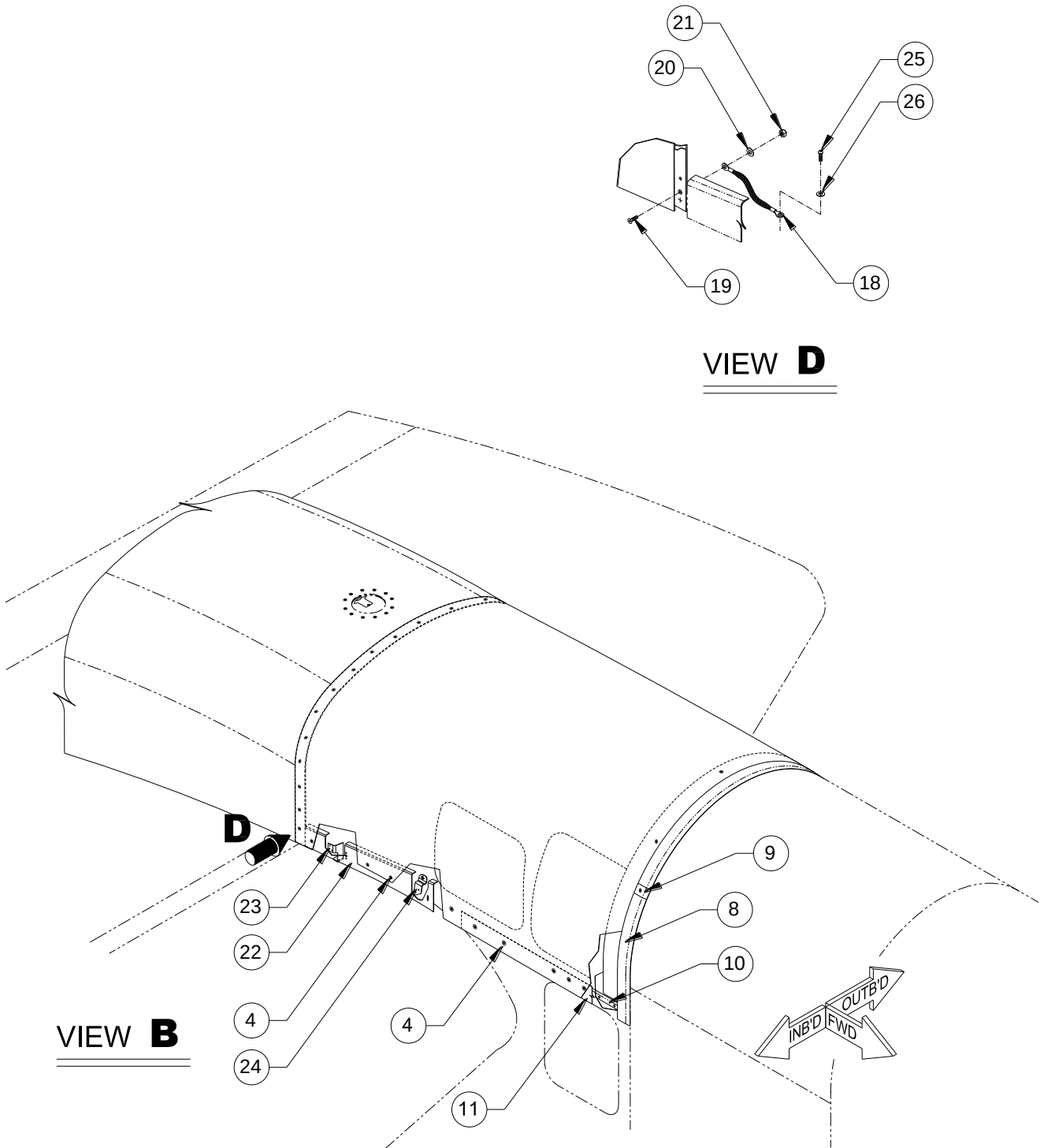
FIGURE 10-12 - SADDLE TANK FAIRINGS (300/B300) SHEET 2 OF 3
