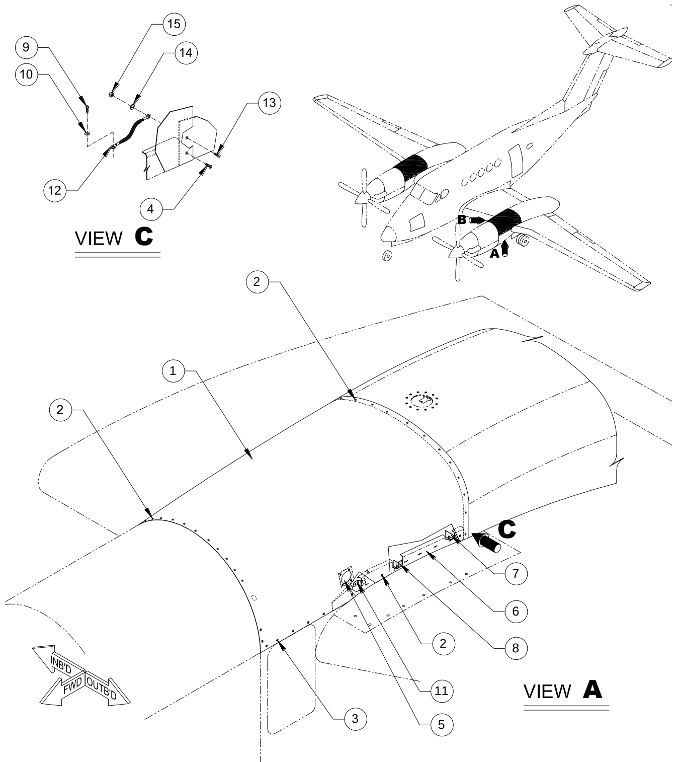
FIGURE 10-11 - SADDLE TANK FAIRINGS (BL-7) SHEET 1 OF 2
